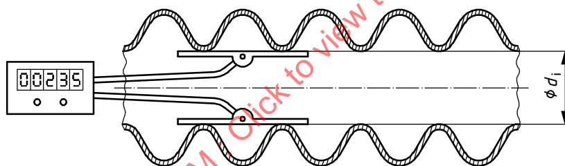
Figure 1 — Example of device for measuring the inside diameter of a corrugated pipe
