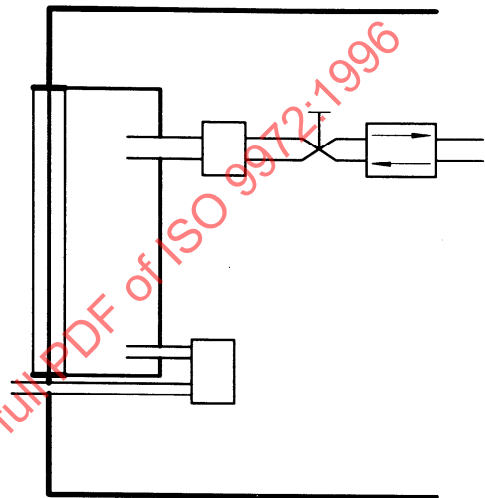
Figure A.2 — Schematic layout of equipment for component airtightness test using a pressurized enclosure
