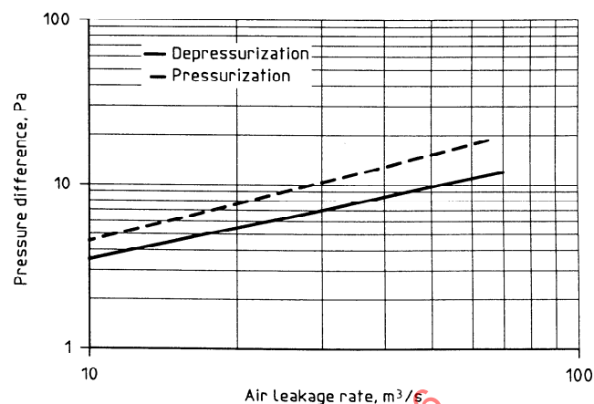
Figure 1 — Example of air leakage graph
