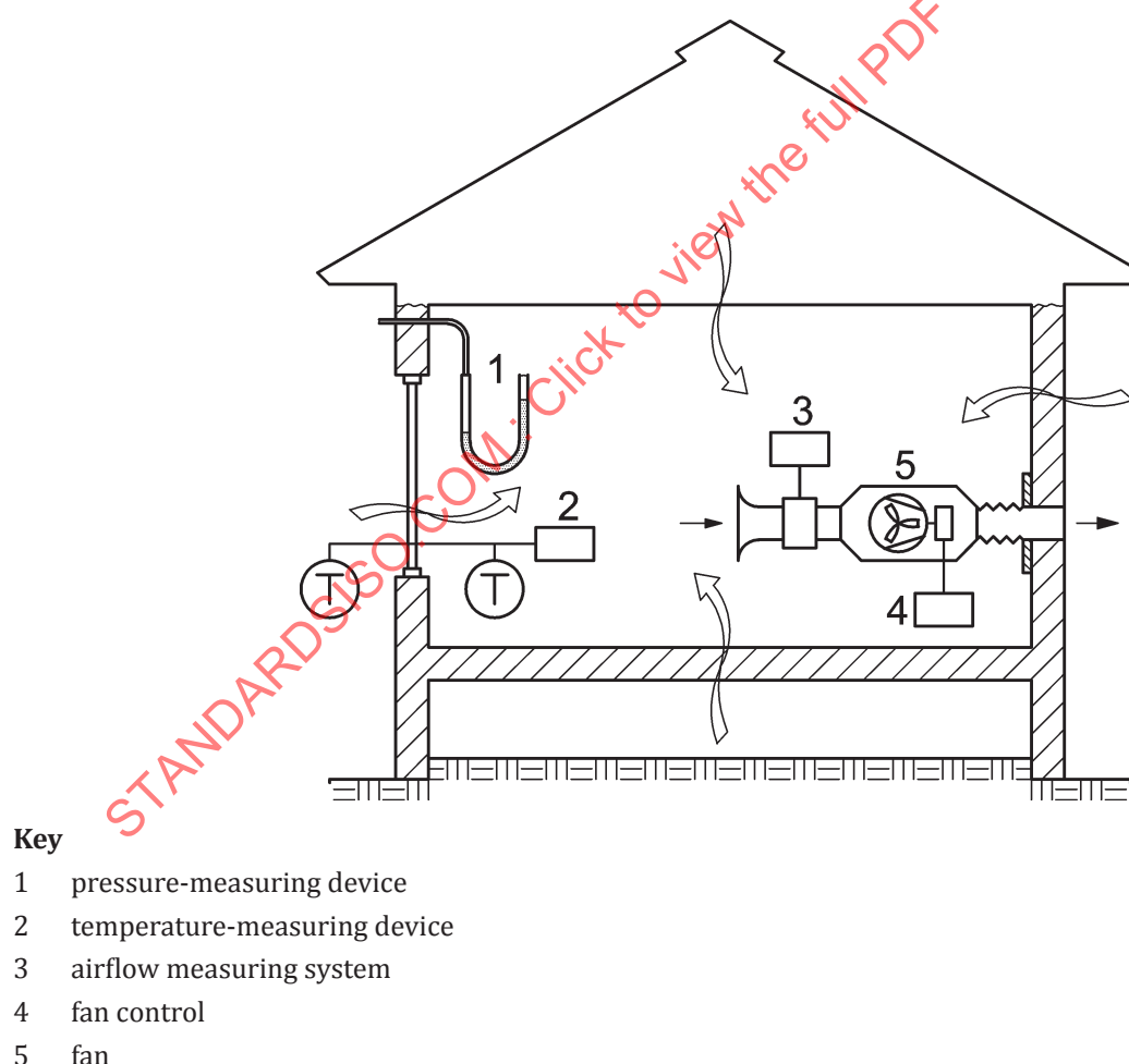
Figure A.1 — Schematic layout of equipment for whole building test
