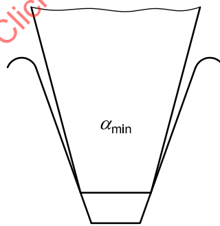
Figure 3 — Fitting of limit gauge in the groove to be checked (good)
