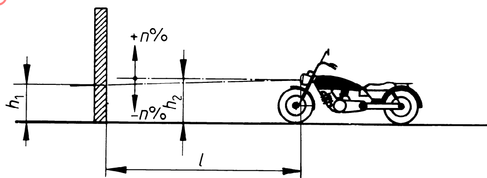
Figure 1 — Dipped beam downward inclination for motorcycle
