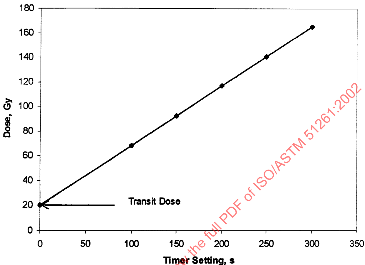
FIG. A2.1 Transit Dose Effect
