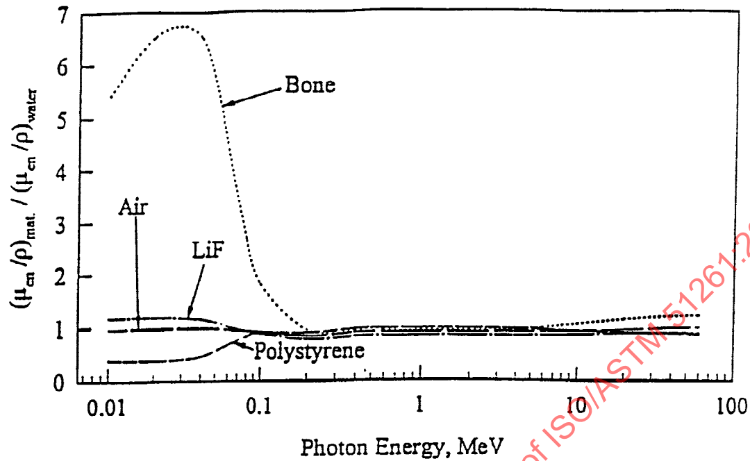
FIG. A1.1 Ratios of Mass Energy Absorption Coefficients
