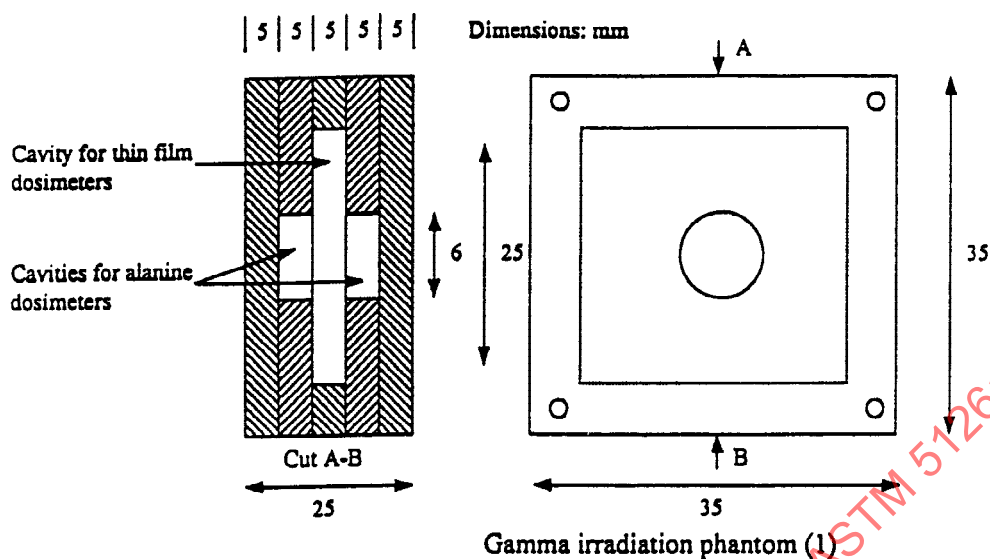
FIG. 1 Example of Calibration Package Allowing Alanine Dosimeters to be Placed on Either Side of Thin Film Routine Dosimeters
