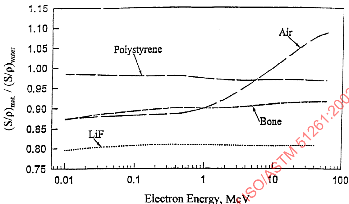
FIG. A1.3 Ratios of Mass Collision Stopping Powers
