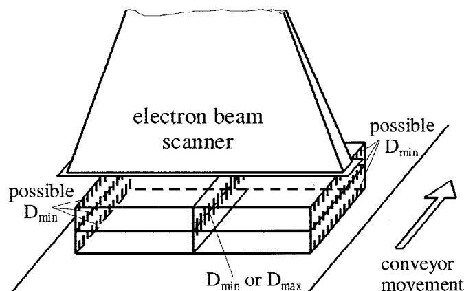
FIG. 5 Regions of D_{\max} and D_{\min} (indicated by hatching) for a rectangular process load after two-sided irradiation using an electron beam
