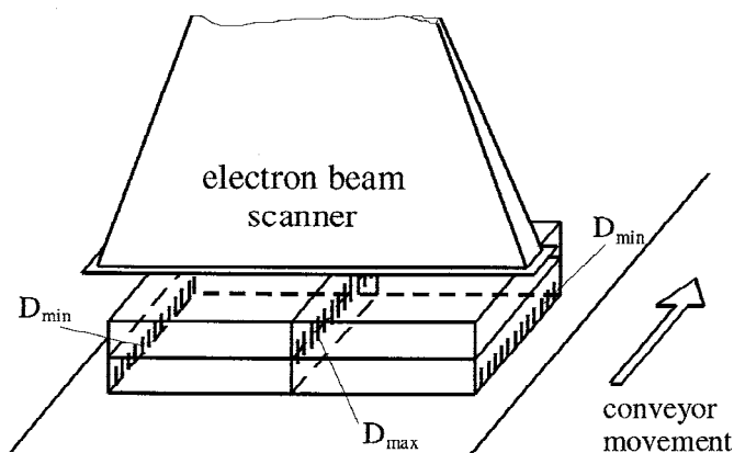
FIG. 4 Regions of D_{\max} and D_{\min} (indicated by hatching) for a rectangular process load after one-sided irradiation using an electron beam
