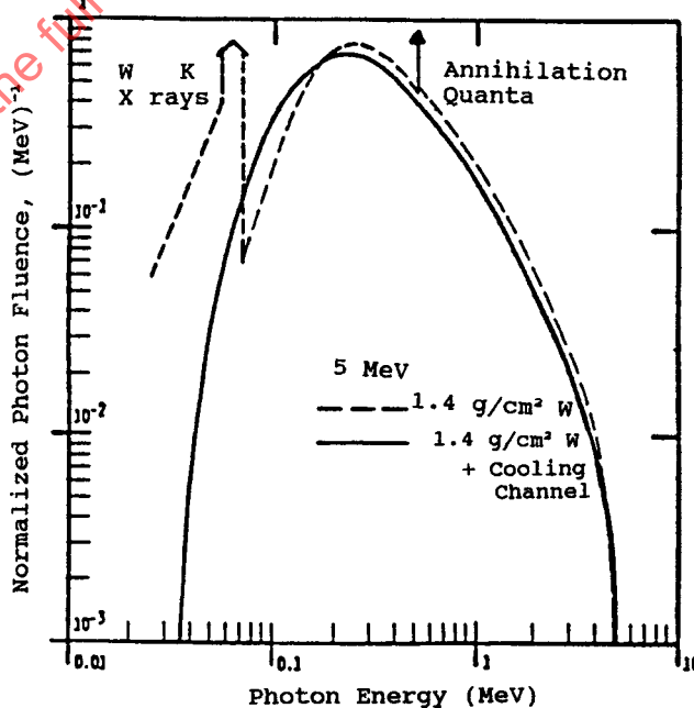
FIG. A1.4 X-ray emission rates from high-Z targets (Fig. E 1 from Ref (88))
