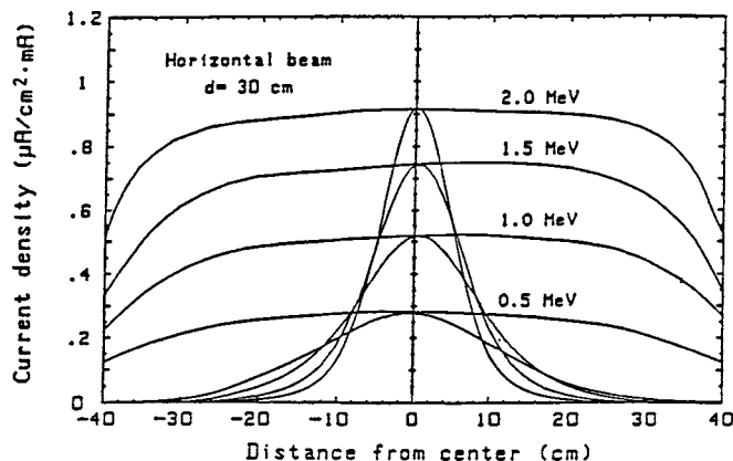
FIG. A1.1 Beam current density distributions along the scan direction (wide curves) and perpendicular to the scan direction (narrow curves) of No. 1 accelerator of JAERI Takasaki (Fig. 2.1 from Ref (73))
