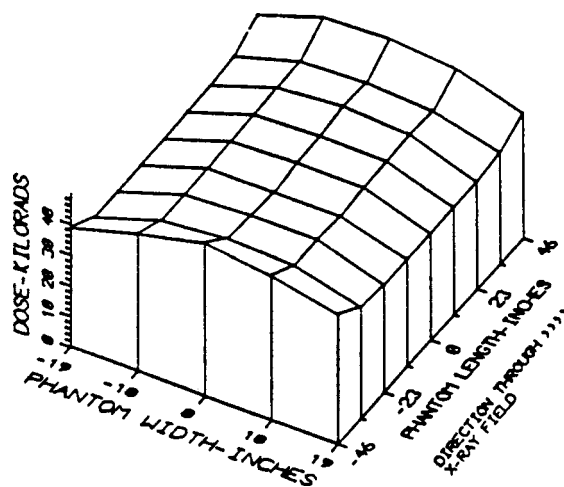
FIG. A1.8 Dose contour map, moving exposure (Fig. 3 from Ref (74))
