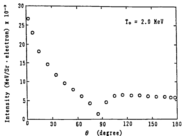
FIG. A1.2 X-ray intensity per 2 MeV electron incident perpendicularly on a tantalum target with thickness of one CSDA electron range as a function of emitting angle calculated by the ETRAN code (Fig. 3.3 from Ref (73))
