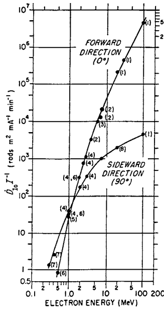
FIG. A1.4 X-ray emission rates from high-Z targets (Fig. E 1 from Ref (76))
