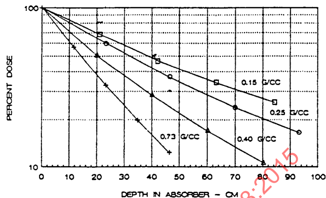
FIG. A1.9 Measured attenuation curves for 5 MeV X-Rays in absorbers of various densities, with moving conveyor and scanning beam (Fig. 5 from Ref (3))
