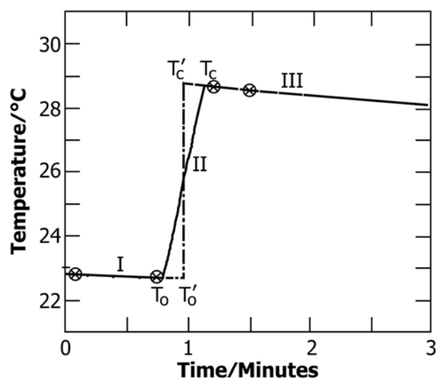
FIG. 4 Example of on-line measurements of a graphite calorimeter (5)
