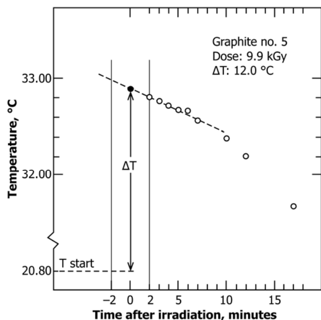
FIG. 3 Example of measurements of temperature of a graphite calorimeter before and after irradiation (7)
