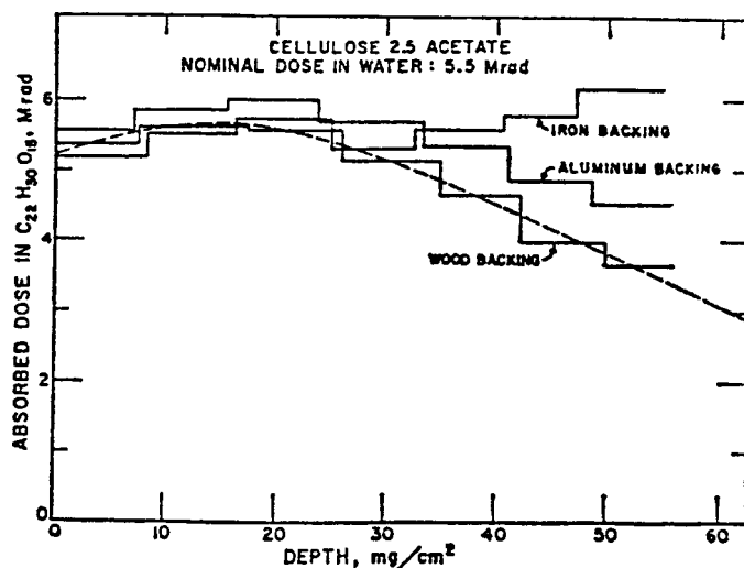
FIG. A2.11 Depth-dose distributions in stacks of cellulose acetate films backed with wood, aluminum, and iron for incident electrons with 400 keV energy (30)
