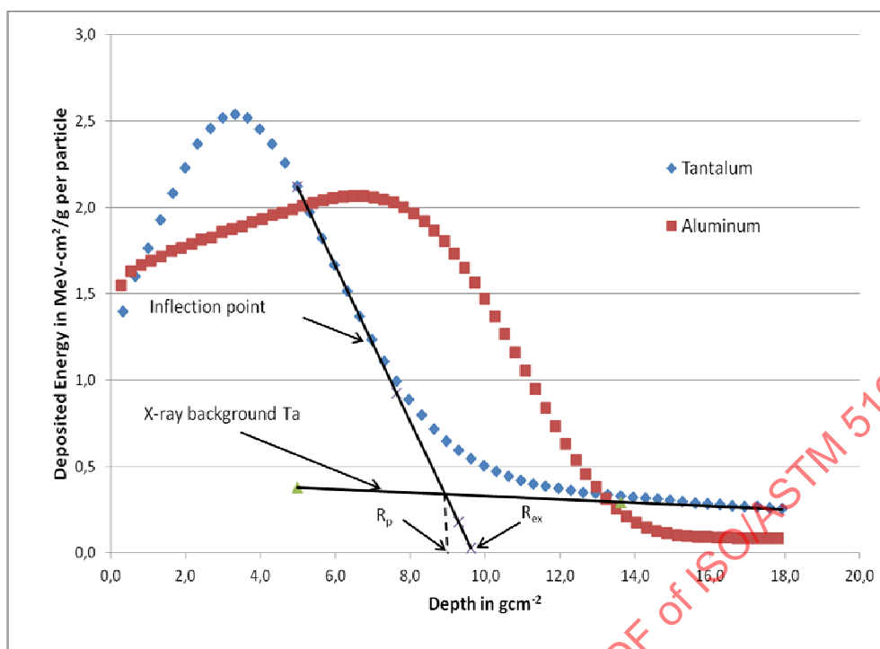
FIG. A2.6 Calculated depth-dose distributions in Al and Ta for normally incident electrons at a monoenergetic energy of 25 MeV using the program ITS3 (19, 24)
