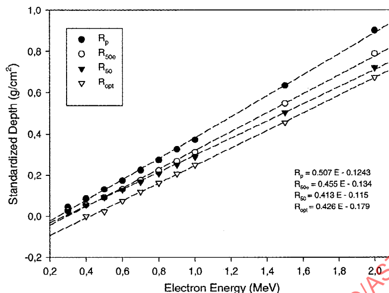
FIG. A2.8 Calculated correlations between incident electron beam energy and optimum thickness R_{opt} , half-value depth R_{50} , half-entrance depth R_{50e} , and practical range R_p for polystyrene using data from Fig. A2.3 and Fig. A2.4 (see Table A4.1)
