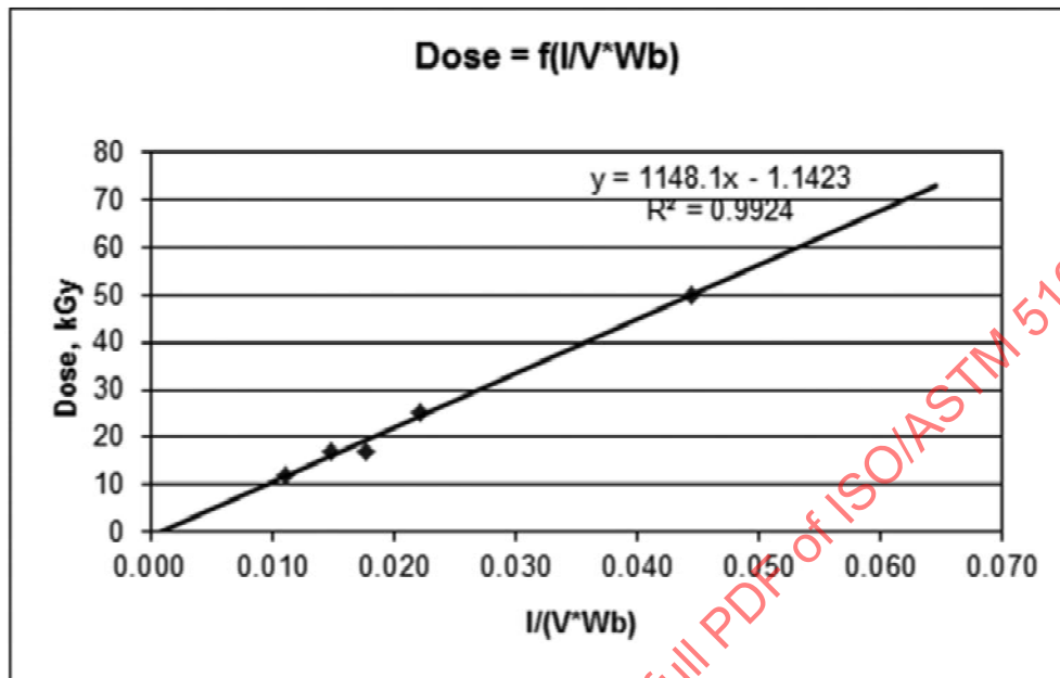
FIG. A5.1 Example of dose as function of average beam current ( I ), conveyor speed ( V ) and beam width ( W_b )
