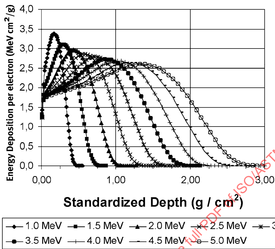
FIG. A2.4 Calculated depth-dose distributions in polystyrene for normally incident electrons at monoenergetic energies from 1.0 to 5.0 MeV using the program ITS3 (19, 20)
