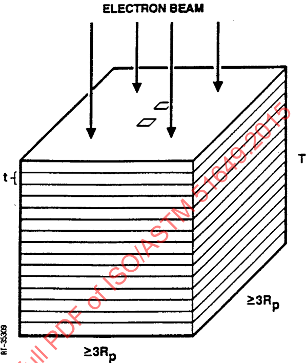
NOTE 1—Plate thickness t \leq R_p/12 and the stack height T \geq 1.5 R_p , where R_p is the anticipated practical range of the electron beam in the stack material. At least two film dosimeters should be placed on the top (shown in drawing) and between the plates along the center of the stack.
