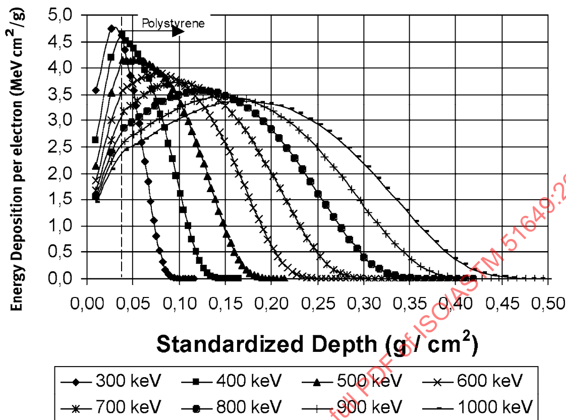
FIG. A2.3 Calculated depth-dose distributions in polystyrene for normally incident electrons at monoenergetic energies from 300 to 1000 keV using the Program ITS3 (19, 20)
