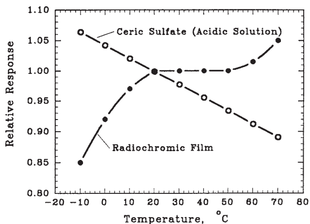
FIG. A2.1 Irradiation temperature dependence
