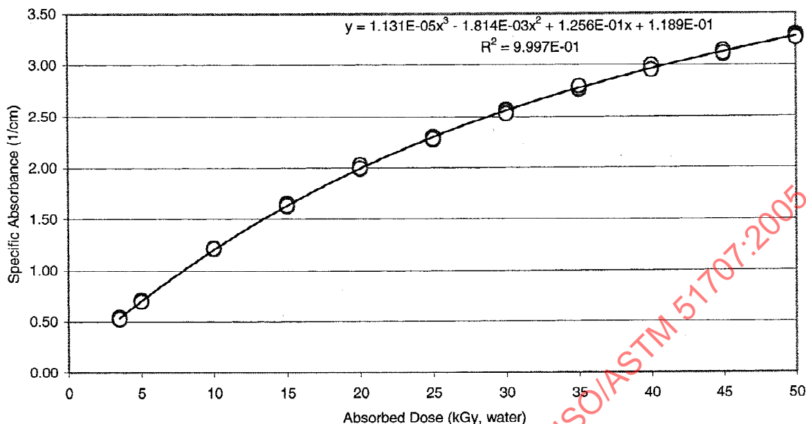
FIG. A4.1 Response curve (3rd order polynomial) for Red 4034 dosimetry data in Table A4.2
