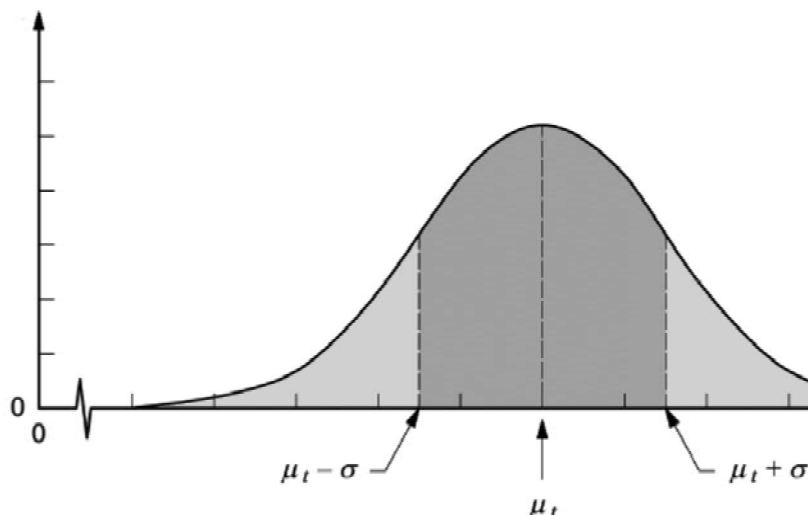
FIG. 1 Normal distribution, also called Gaussian or “bell curve”, the most important continuous random distribution (JCGM 100:2008)
