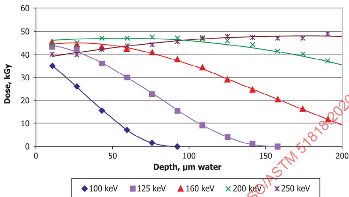
FIG. A1.7 Examples of measurements of depth-dose distributions at the same electron beam facility, but at different beam energies
