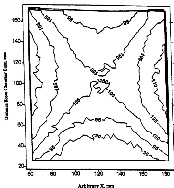
FIG. 1 Example of two-dimensional dose mapping results normalized to a central dose of 100 %
