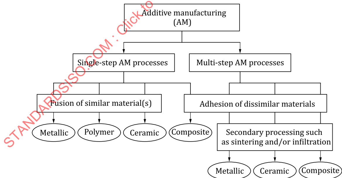
Figure A.1 — Single-step and multi-step AM process principles
