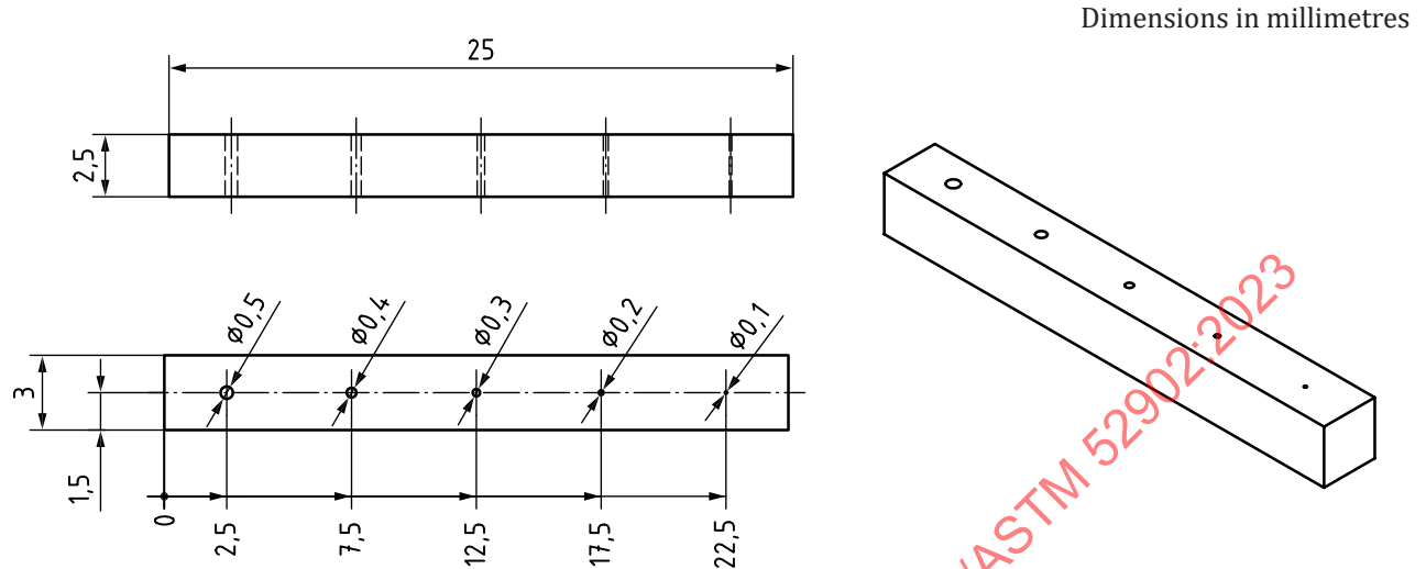
Figure 6 — Engineering drawing of medium resolution holes feature
