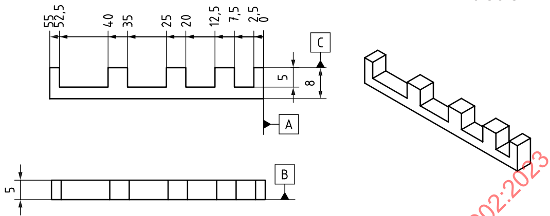
Figure 1 — Engineering drawing of linear test artefacts
