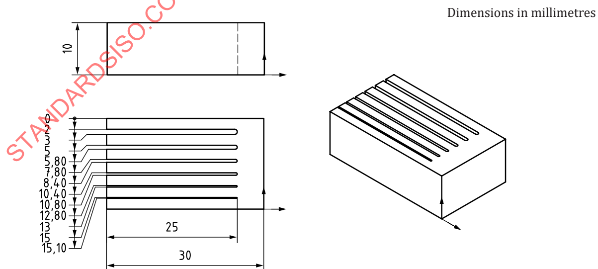
Figure 9 — Engineering drawing of medium resolution slots feature with 10,0 mm high walls
