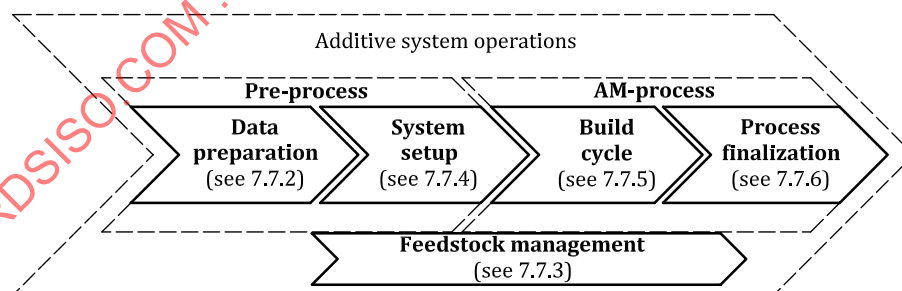
Figure 4 — Elements of additive system operations
