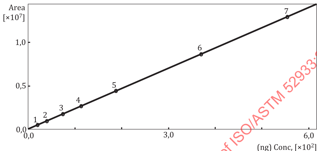
Figure 4 — Example of creating a calibration curve
