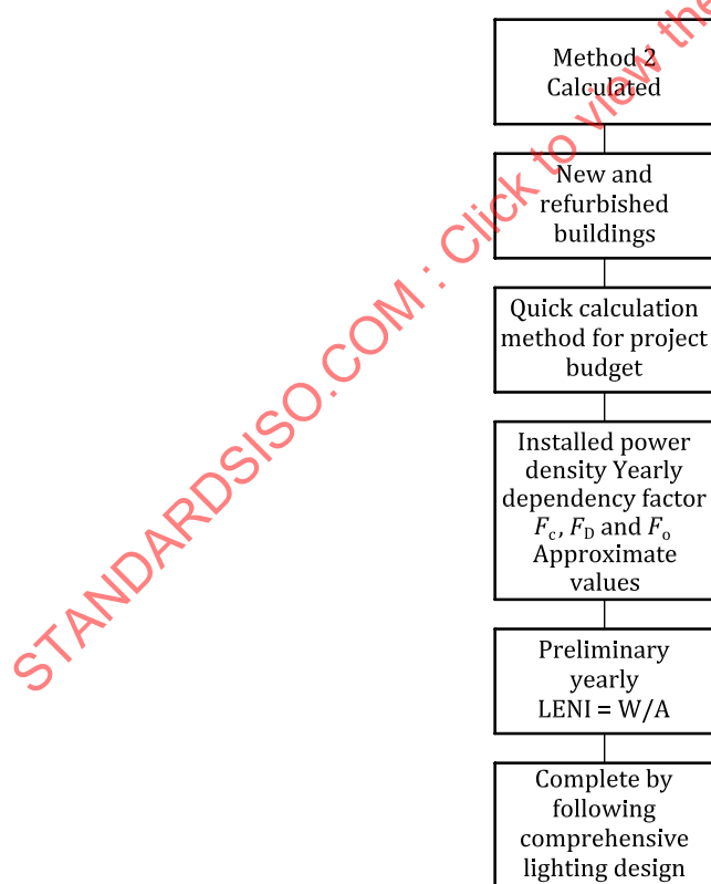
Figure 5 — Flow diagram for quick method of lighting energy calculation
