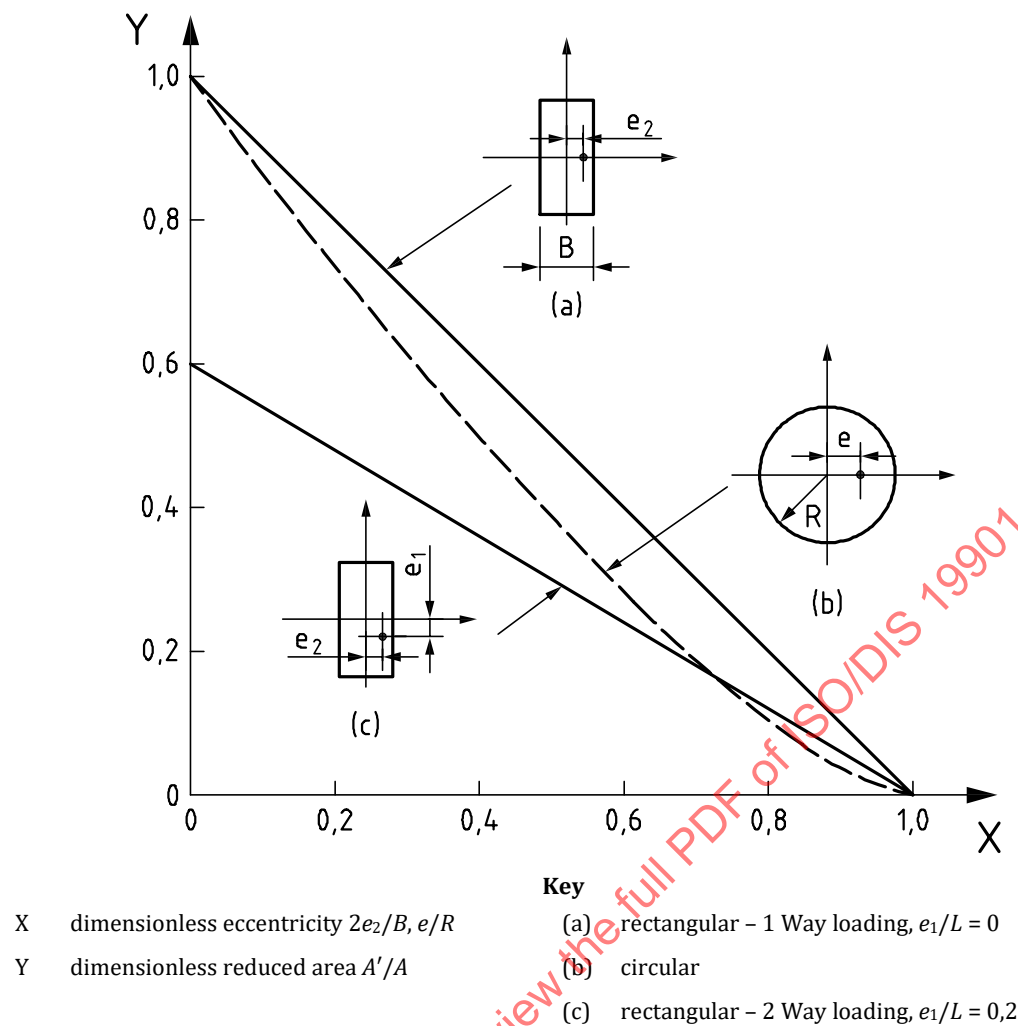
Figure A.2 — Area reduction factors for eccentrically loaded shallow foundations
