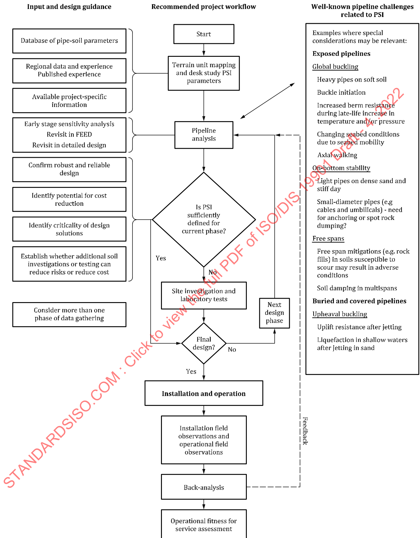
Figure A.22 — Example of pipe-soil interaction workflow during a project (based on Reference [111])
