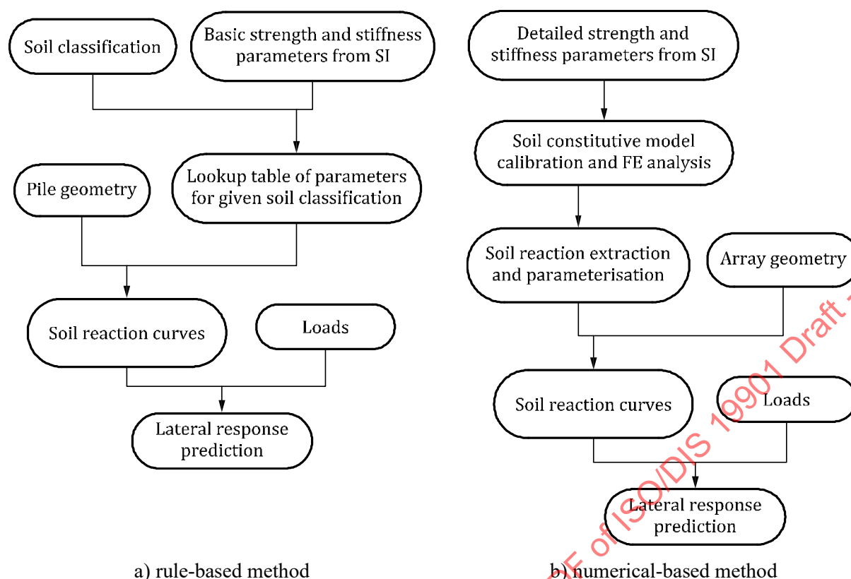
Figure A.17 — Application modes for the design method
