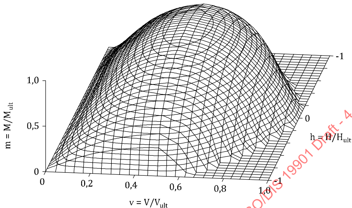
Figure A.6 — Yield surface for undrained conditions for a surface foundation with zero-uplift capacity along the foundation-soil interface [332]
