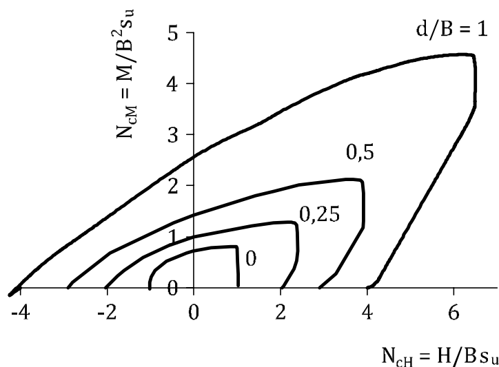
Figure A.8 — Change in shape of yield surface for undrained conditions with foundation embedment d/B [153]
