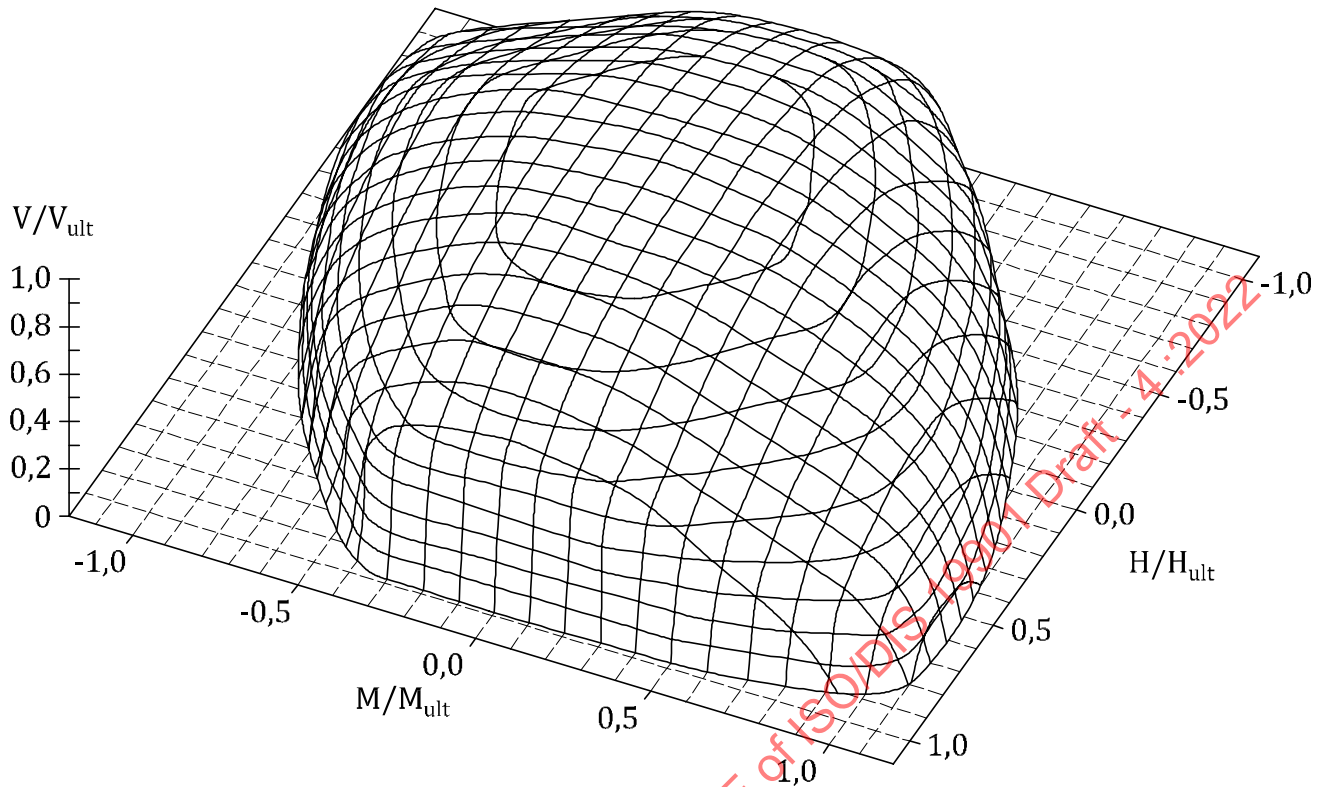
Figure A.7 — Yield surface for undrained conditions for a surface foundation with unlimited-uplift capacity along the foundation-soil interface [55]
