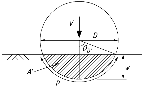
Figure A.24 — Pipeline embedment notation
