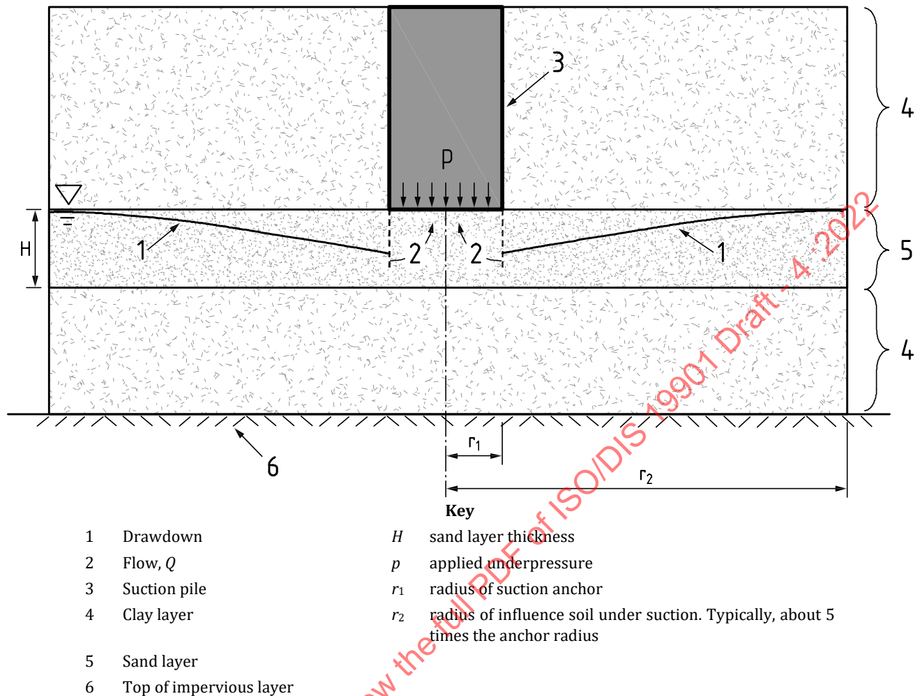
Figure A.21 — Illustration of water flow in sand layer below a suction pile under tension
