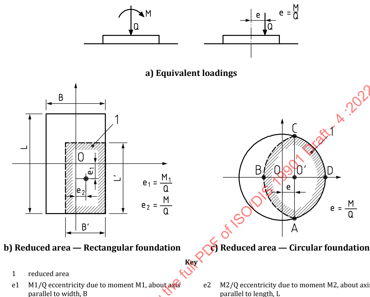
Figure A.1 — Definition of effective area for various foundation geometries
