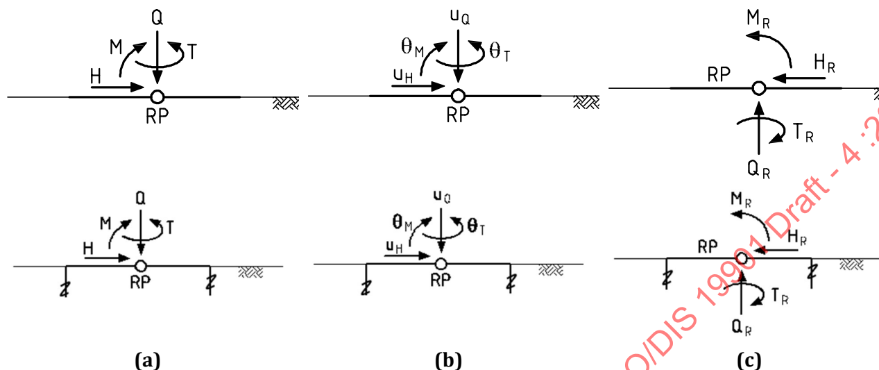
Figure 7 — Sign conventions, nomenclature and reference point for analysis of shallow and intermediate foundation (a) actions, (b) displacements and rotations, (c) seabed resistance
