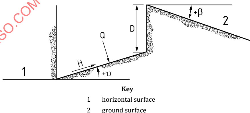
Figure A.3 — Definitions for inclined base and seafloor surface [62]
