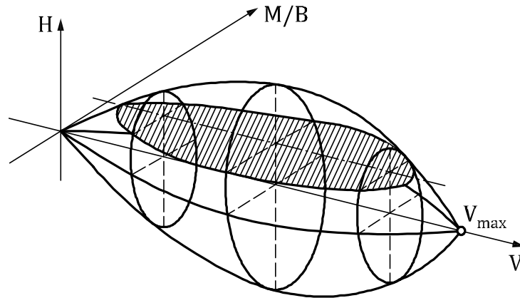
Figure A.9 — Yield surface for drained conditions for a surface foundation [68]
