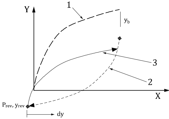
Figure A.19 a) Degrading p-y model
