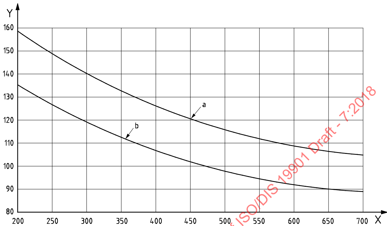
Key X power/propeller disk area, kW/m 2 Y specific thrust, N/kW a Optimum value b Low value NOTE Power delivered to the propeller per unit propeller area.
