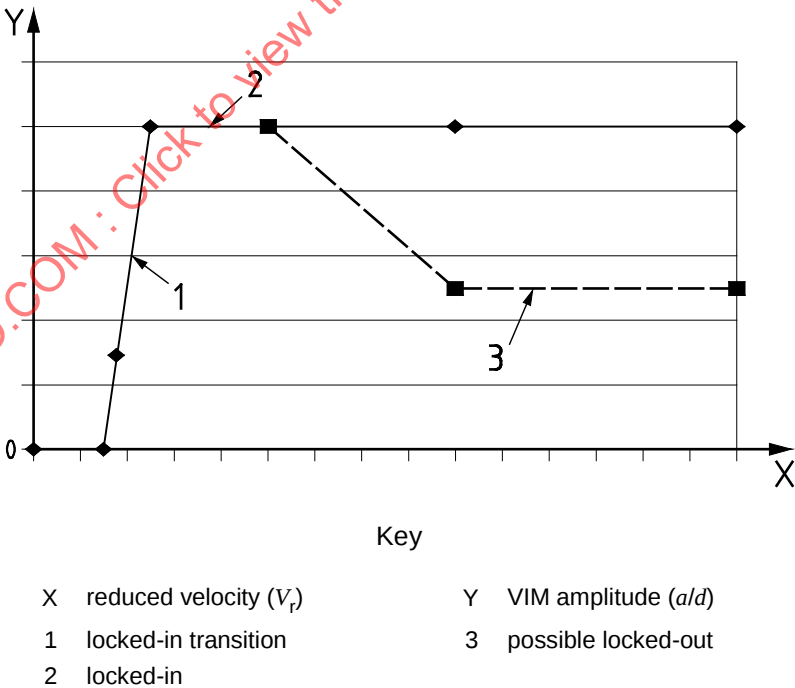
Figure A 11 — Example VIM amplitude vs. reduced velocity
