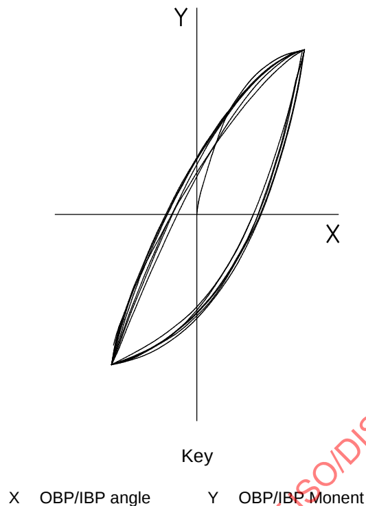
Figure A 18 Interlink moment vs angle
