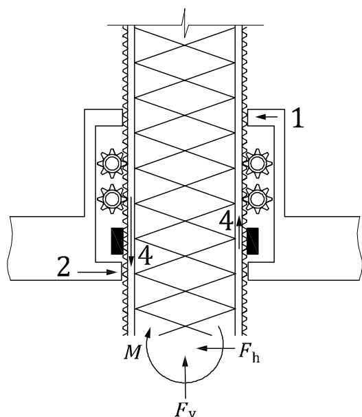
c) Jacking system with fixation system
