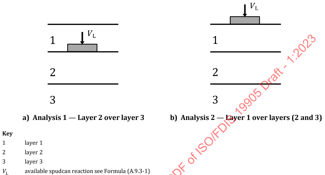
Figure A.9.3-13 — Spudcan bearing capacity analysis — Three-layer case
