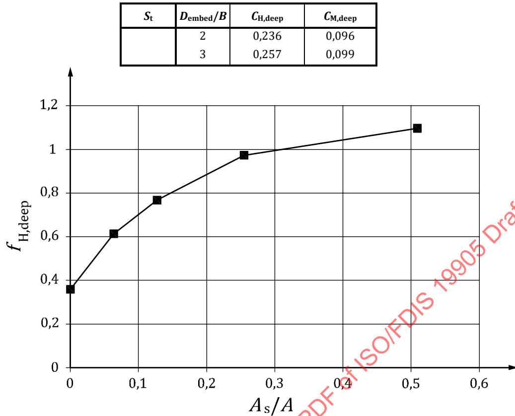
Figure A.9.3-15 — Effect of spudcan aspect ratio A_s/A on C_{H,\text{deep}} [after Zhang et al. (2012b) [220] ]
