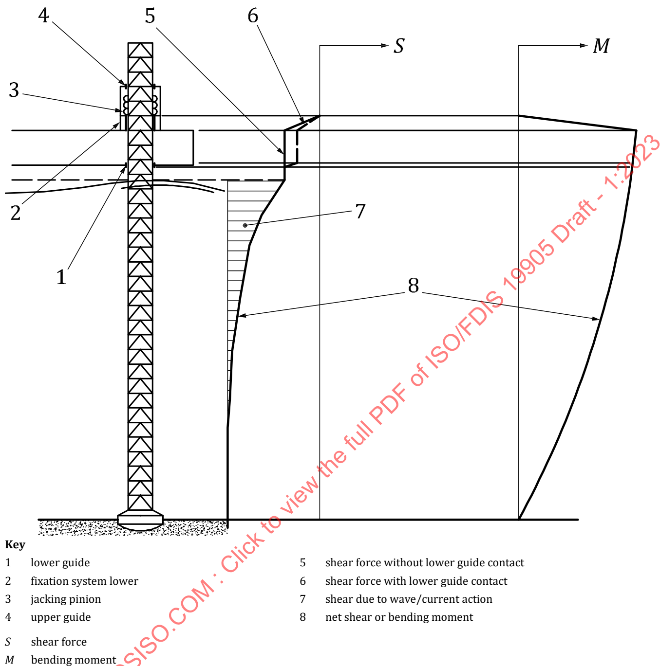
Figure A.8.5-3 — Complete leg shear force and bending moment — Jack-ups with a fixation system
