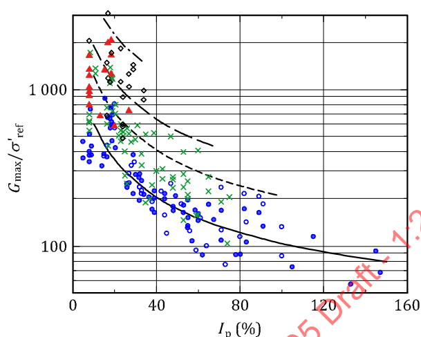
b) G_{\max} normalized with respect to reference effective stress
