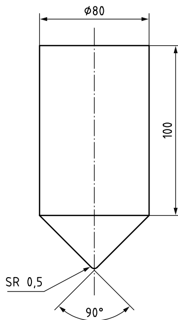
Figure 1 — Test cone
