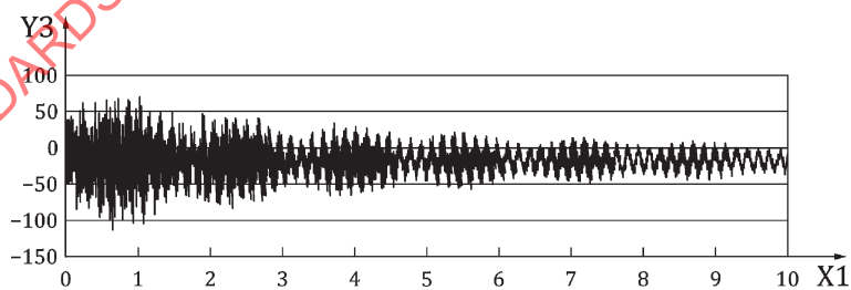
c) Short circuit fault – Stress vs time for two rotor locations
