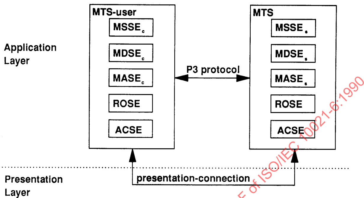
Figure 1 MTS Access Protocol Model
