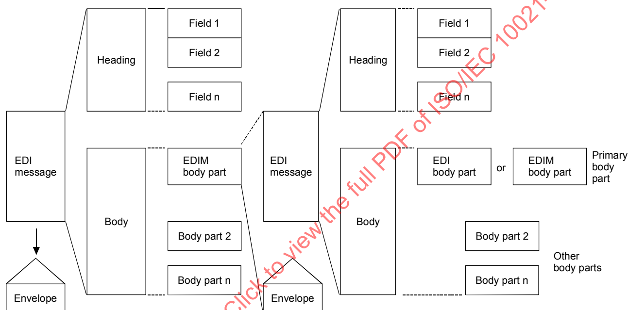
Figure 6 – Forwarding
