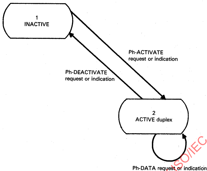
Figure 6 — State transition diagram for Duplex Mode with Activation/Deactivation
