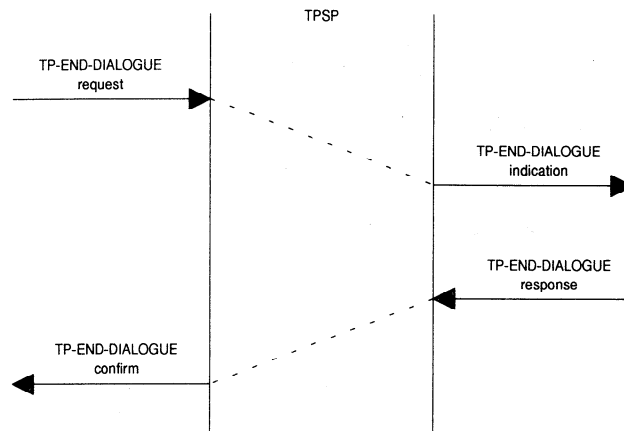
Figure 4 - Confirmed END-DIALOGUE sequence of primitives
