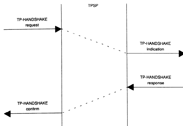
Figure 11 - TP-HANDSHAKE sequence of primitives
