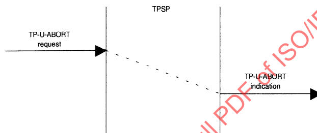
Figure 7 - TP-U-ABORT sequence of primitives
