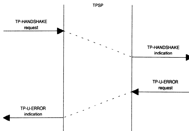
Figure 6 - TP-U-ERROR as the negative confirmation to a handshake service
