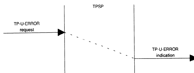
Figure 5 - TP-U-ERROR sequence of primitives
