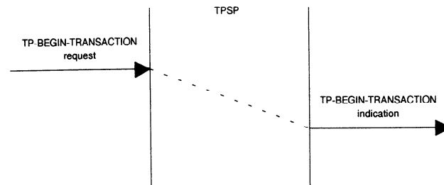
Figure 13 - TP-BEGIN-TRANSACTION sequence of primitives
