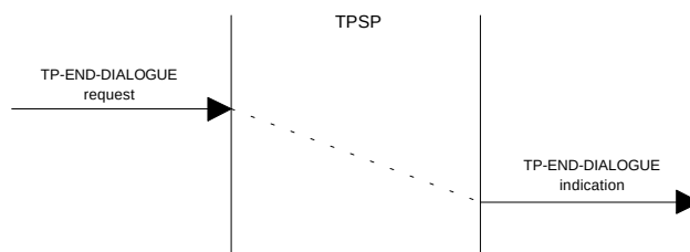
Figure 4 - Unconfirmed TP-END-DIALOGUE sequence of primitives
