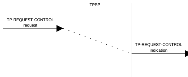
Figure 11 - TP-REQUEST-CONTROL sequence of primitives
