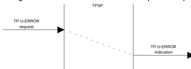
Figure 6 - TP-U-ERROR sequence of primitives
