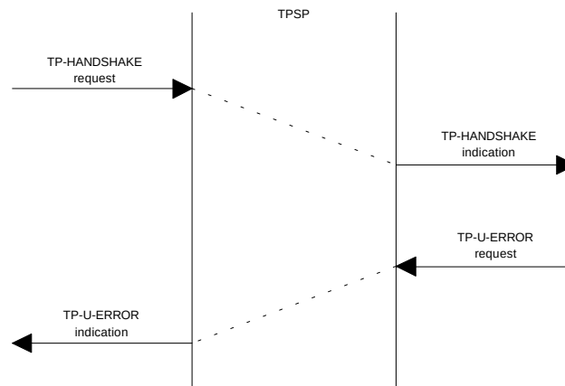
Figure 7 - TP-U-ERROR as the negative confirmation to a handshake service
