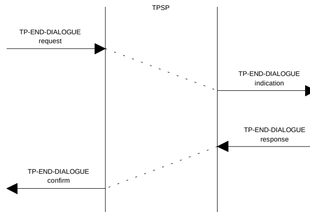
Figure 5 - Confirmed END-DIALOGUE sequence of primitives
