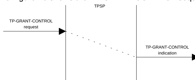
Figure 10 - TP-GRANT-CONTROL sequence of primitives
