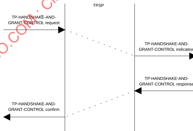
Figure 13 - TP-HANDSHAKE-AND-GRANT-CONTROL sequence of primitives
