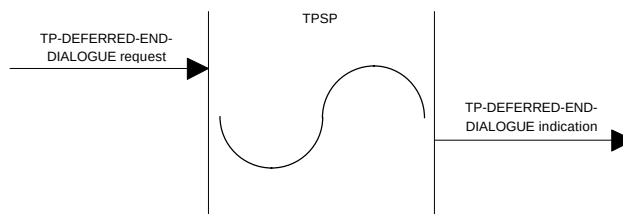
Figure 15 - TP-DEFERRED-END-DIALOGUE sequence of primitives
