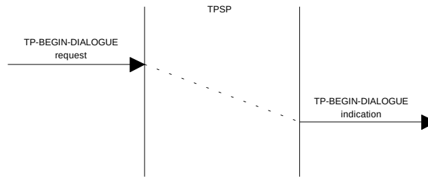
Figure 2 - Unconfirmed TP-BEGIN-DIALOGUE sequence of primitives
