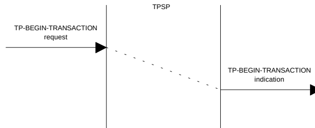
Figure 14 - TP-BEGIN-TRANSACTION sequence of primitives
