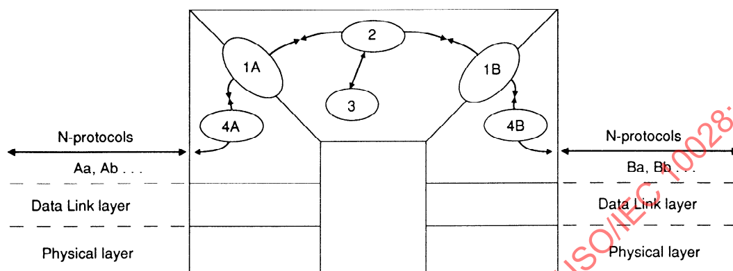
Figure 1 — Intermediate-system model
