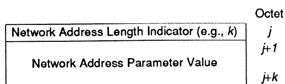
Figure 1 — Network Address Parameter
