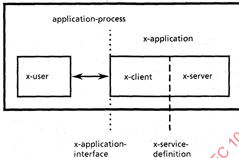
Figure D.1 – Non-distributed Office Application
