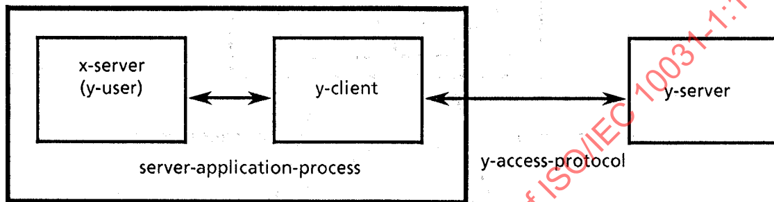
Figure D.7 – A Server as a User of Another Server
