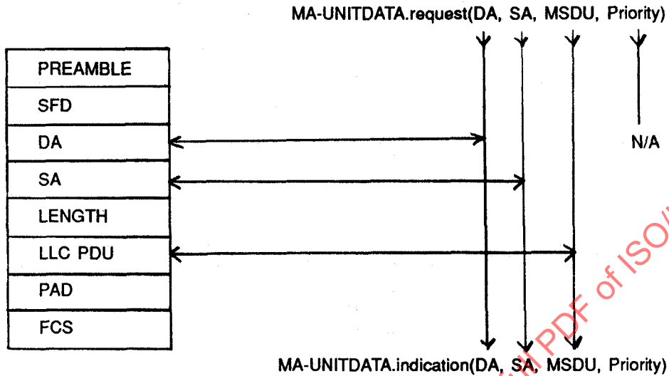
Figure A.1 - Mapping of MAC Service primitives to/from ISO/IEC 8802-3 MAC frames
