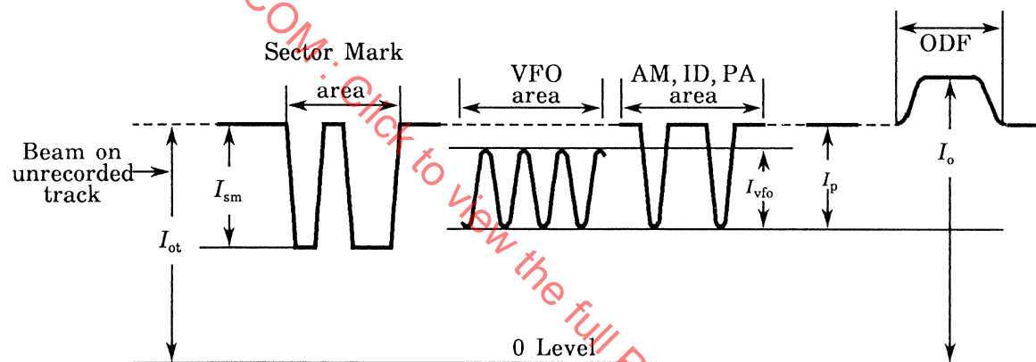
Signals from Headers in Channel 1
