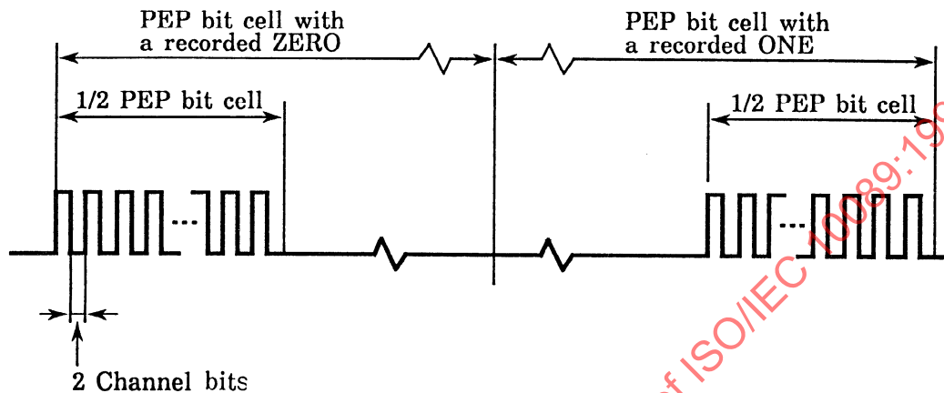
Figure 16 - Example of phase-encoded modulation in the PEP Zone
