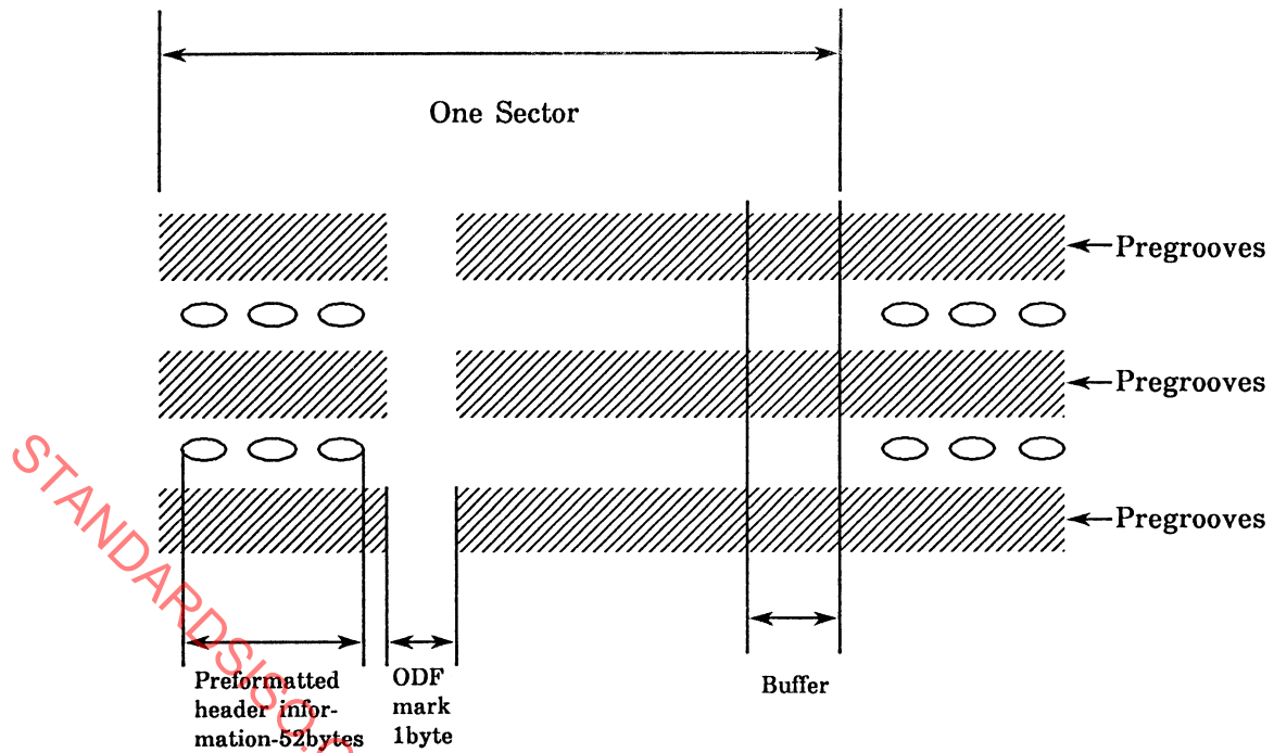
Figure 20 - Example of a sector with Offset Detection Flag for on-land recording (schematic)
