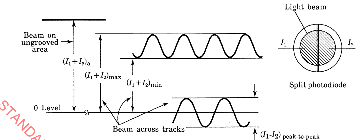
Signals from grooves in the tracking channel
