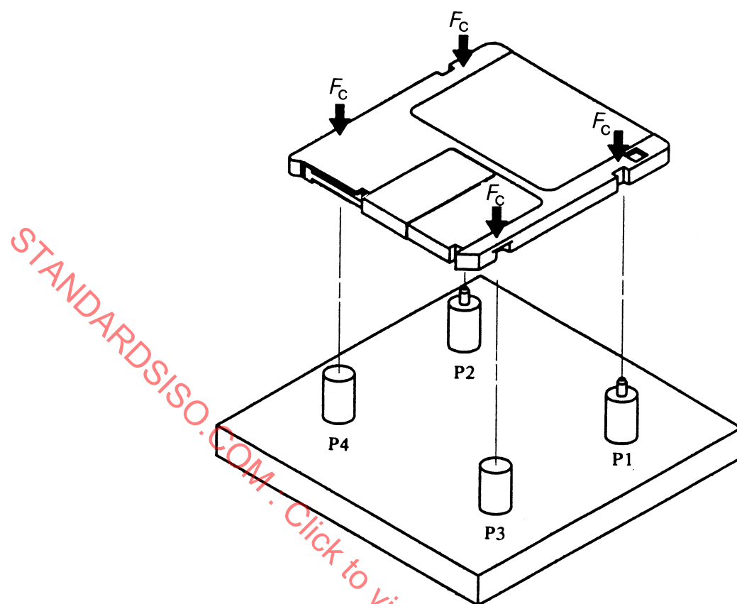
Figure B.1 - Compliance gauge
