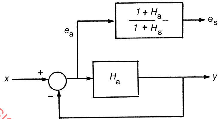
Figure C.4 - Implementation of a Reference Servo by changing the tracking error of the actual servo
