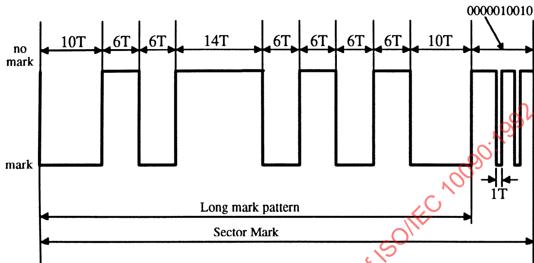
Figure 16 - Pattern of the Sector Mark
