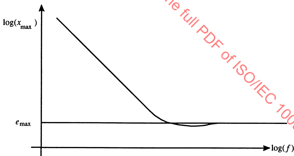
Figure C.1 - Maximum allowed amplitude of a single, sinusoidal track deviation
