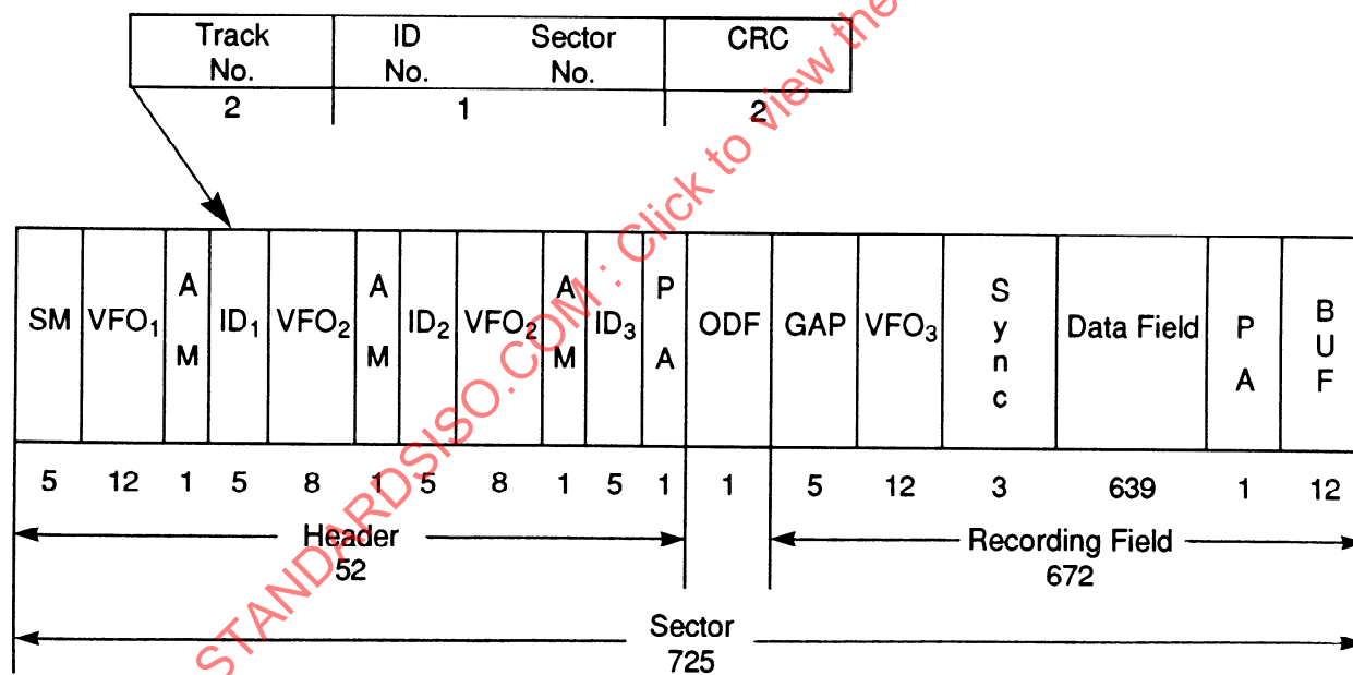
Figure 15 - Sector format
