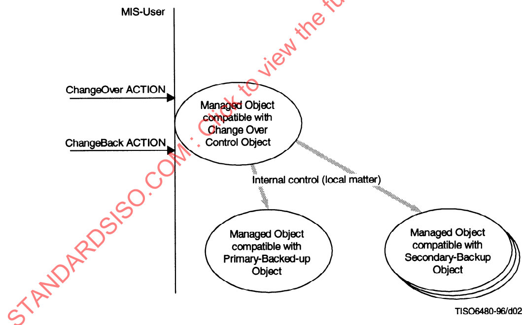
Figure 2 – Change over function model
