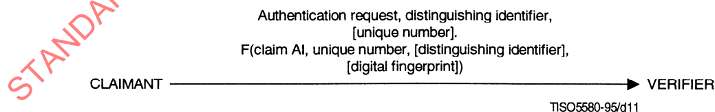
Figure 11 – Sub-class 3 – Unique number mechanism
