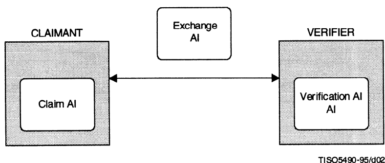
Figure 2 – Authentication without a Trusted Third Party
