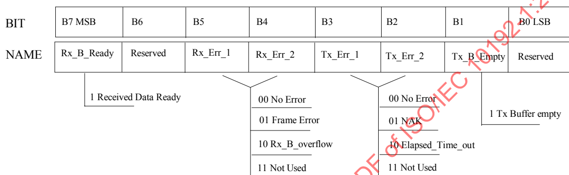
Figure 9 – Status register
