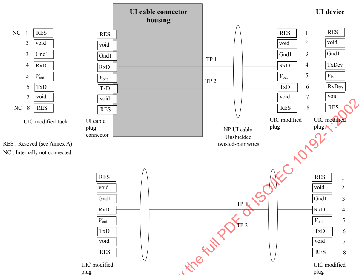
Figure 3 – NP UI cable
