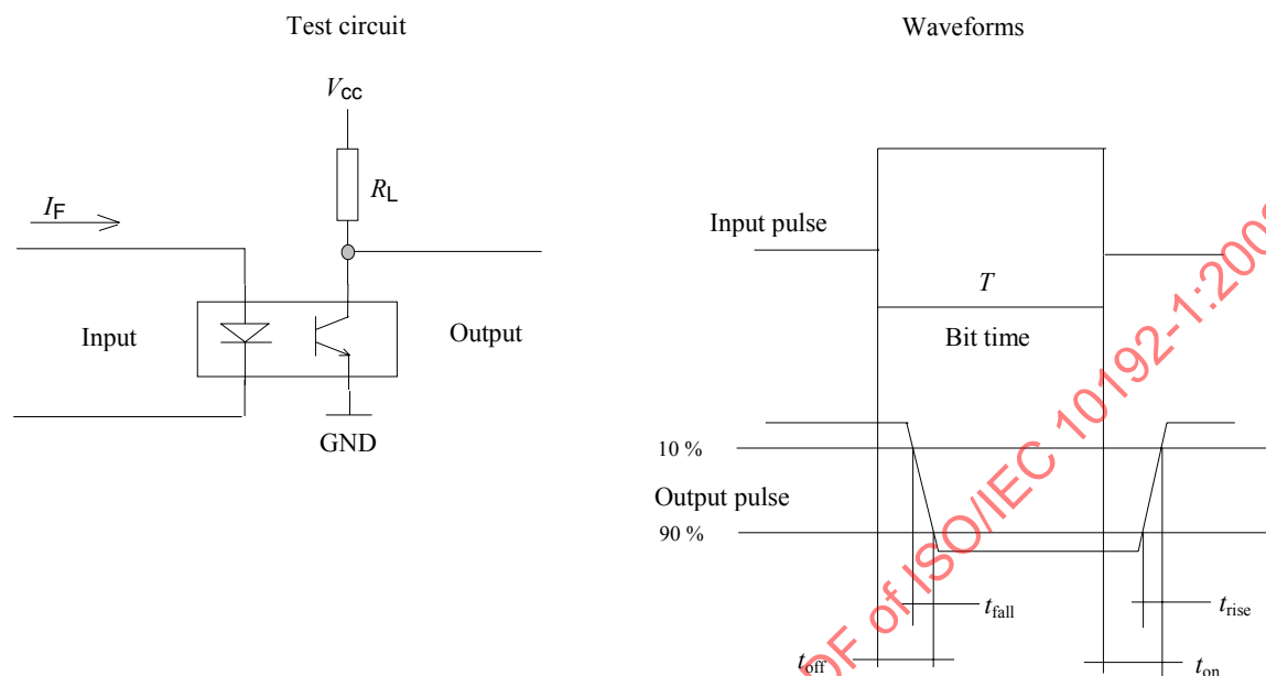
Figure 6 – Test circuit for timing characteristics of optocouplers
