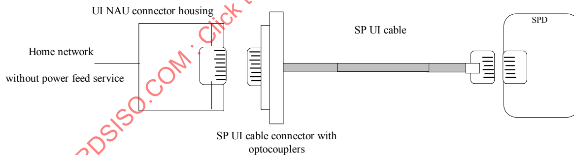
Figure 5 – Connection of an SPD to a home control network that does not provide power
