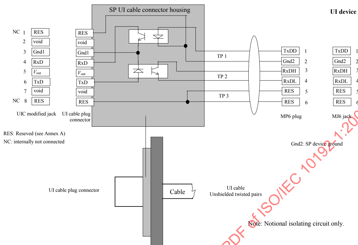
Figure 4 – SP UI cable
