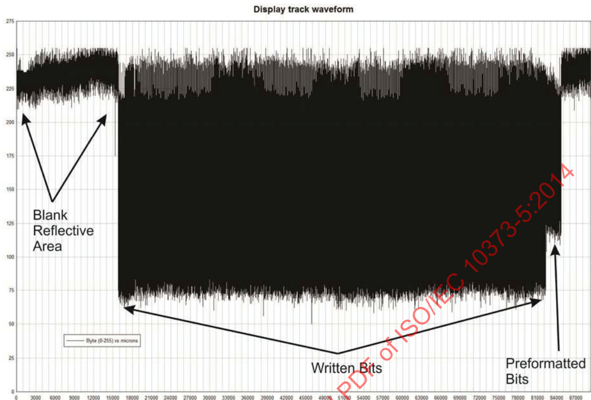
Figure 6 — Full wave scan of written card
