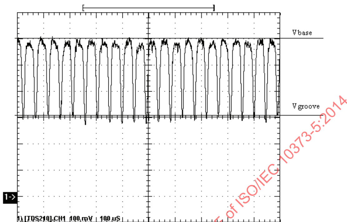
Figure 9 — Track guide contrast
