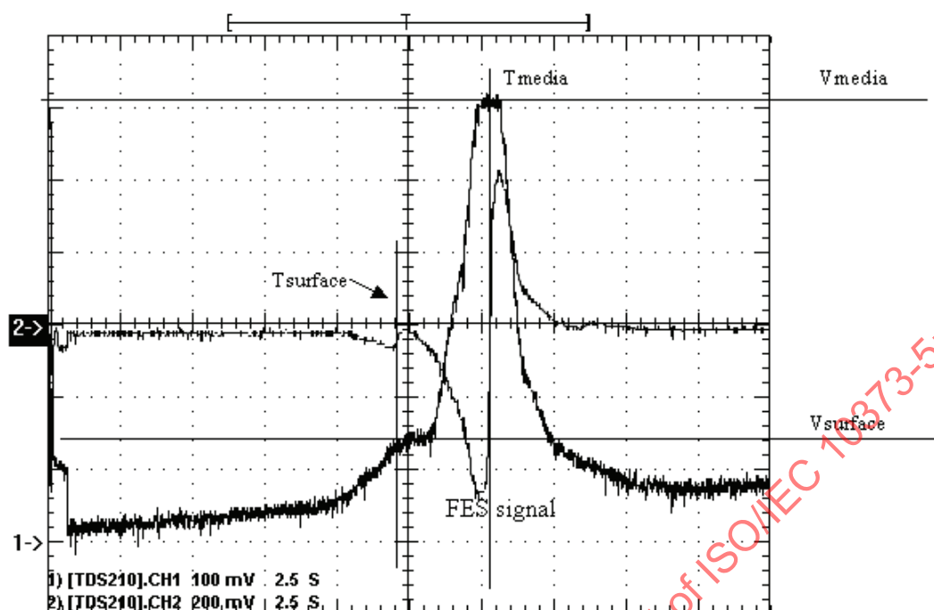
Figure 7 — Focus sweep waveform
