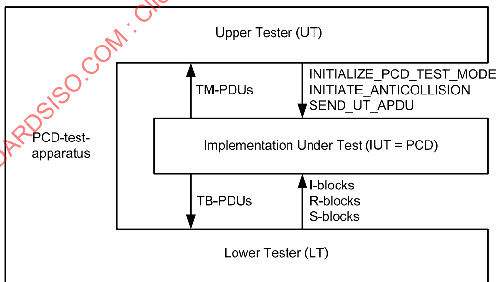
Figure H.1 — Conceptual tester architecture
