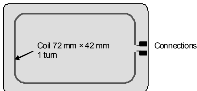
Figure 1 — Calibration coil
