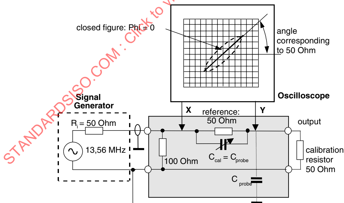
Figure B.1 — Calibration set-up (Step 1)
