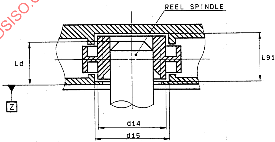
Figure 17 - Interface with the drive spindle
