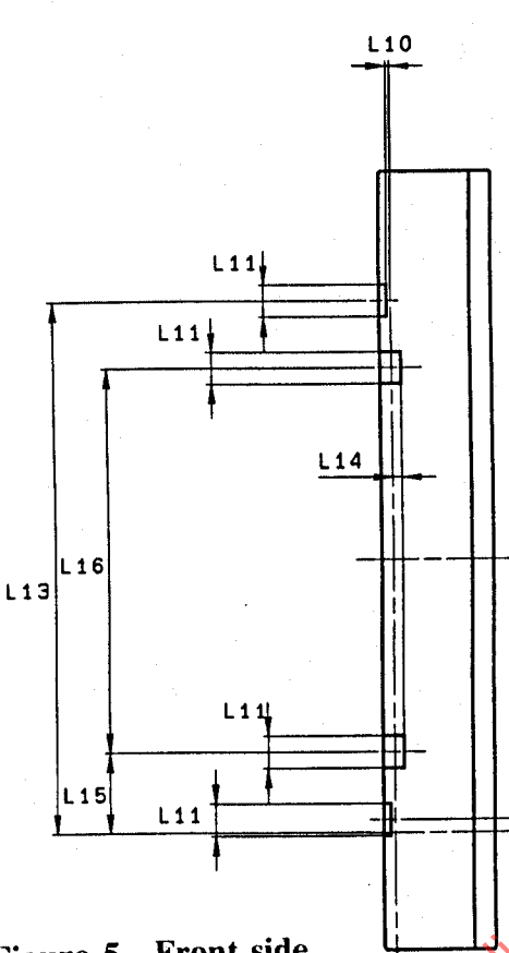
Figure 5 - Front side, lid closed
