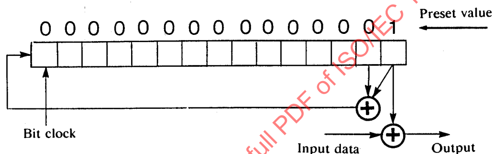
Figure 28 - Shift Register
