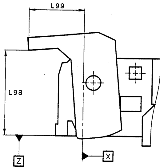
Figure 20 - Minimum position of the lid for which the hubs are completely unlocked
