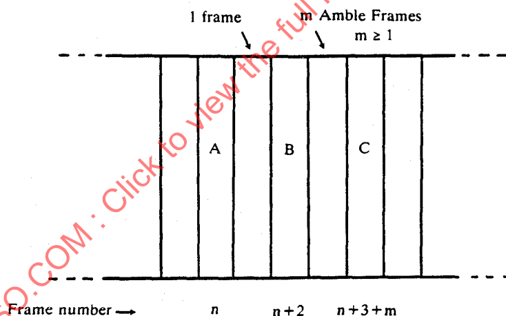
Figure 48 - Appending rules
