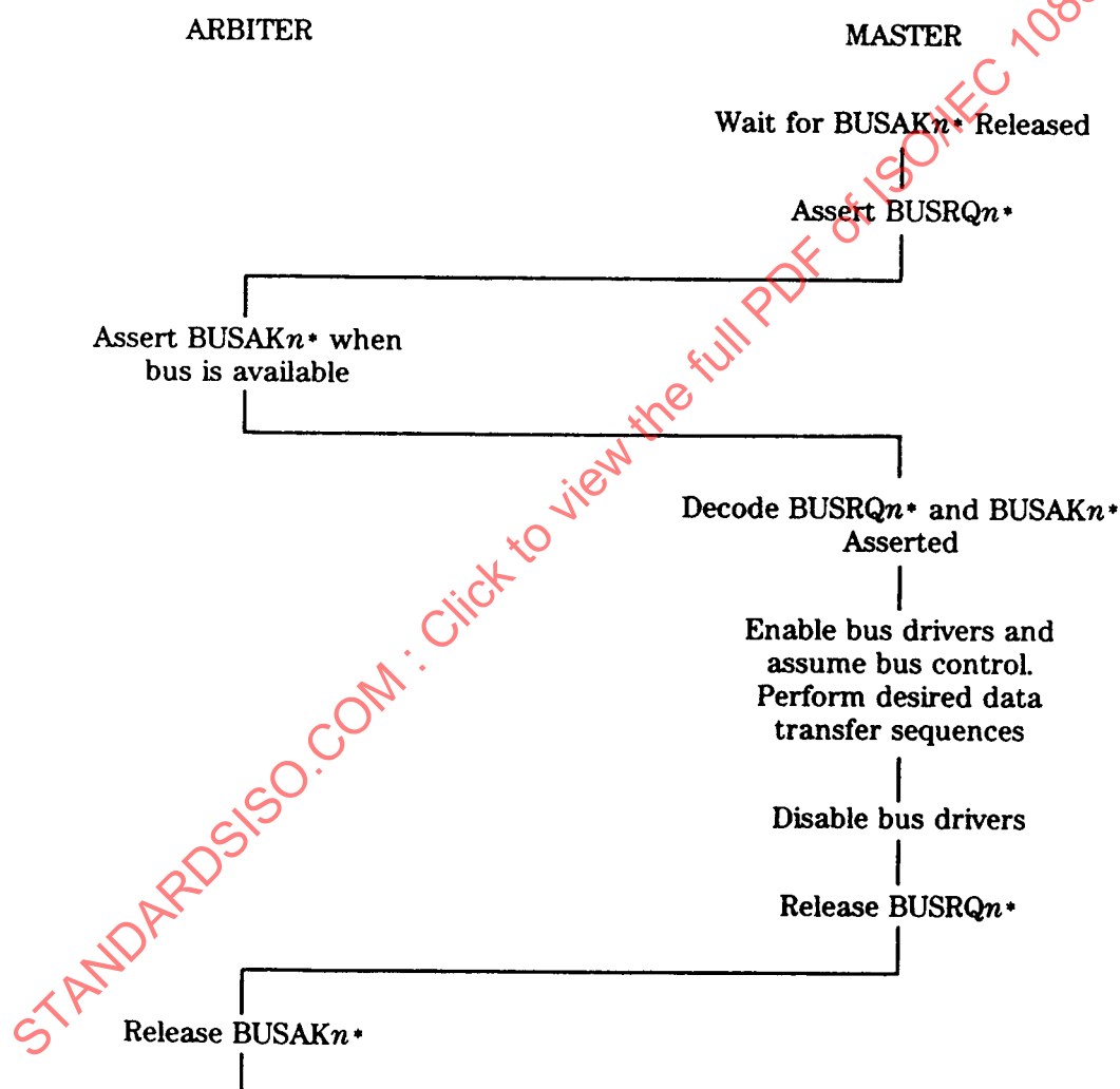
Figure 4 – Control transfer flow diagram
