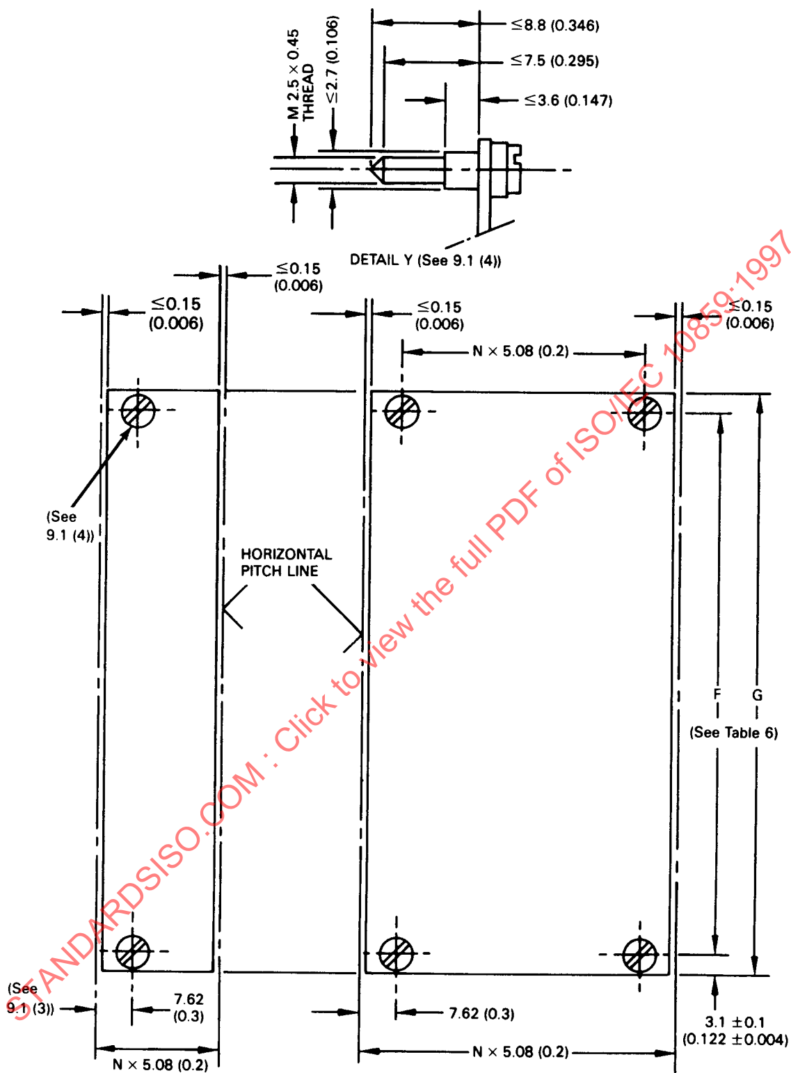
Figure 16 – Filler panels
