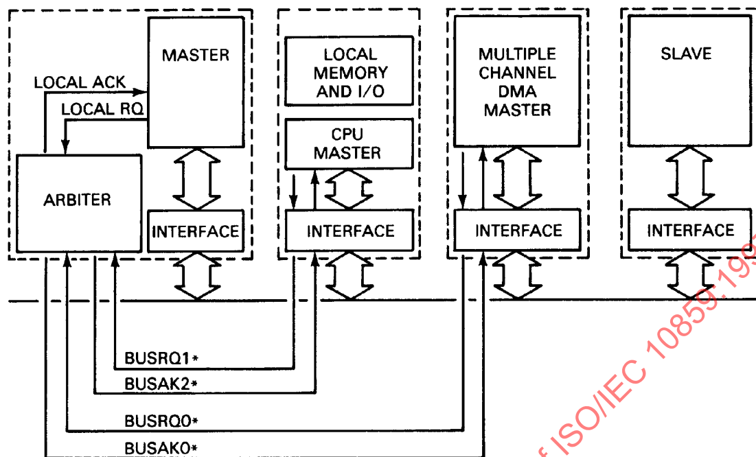
Figure 5 – Example of multiple master implementation
