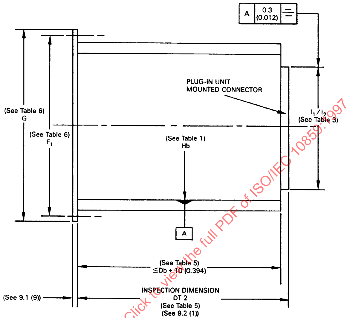
Figure 23 – Box type, box/board type plug-in unit, single height side view
