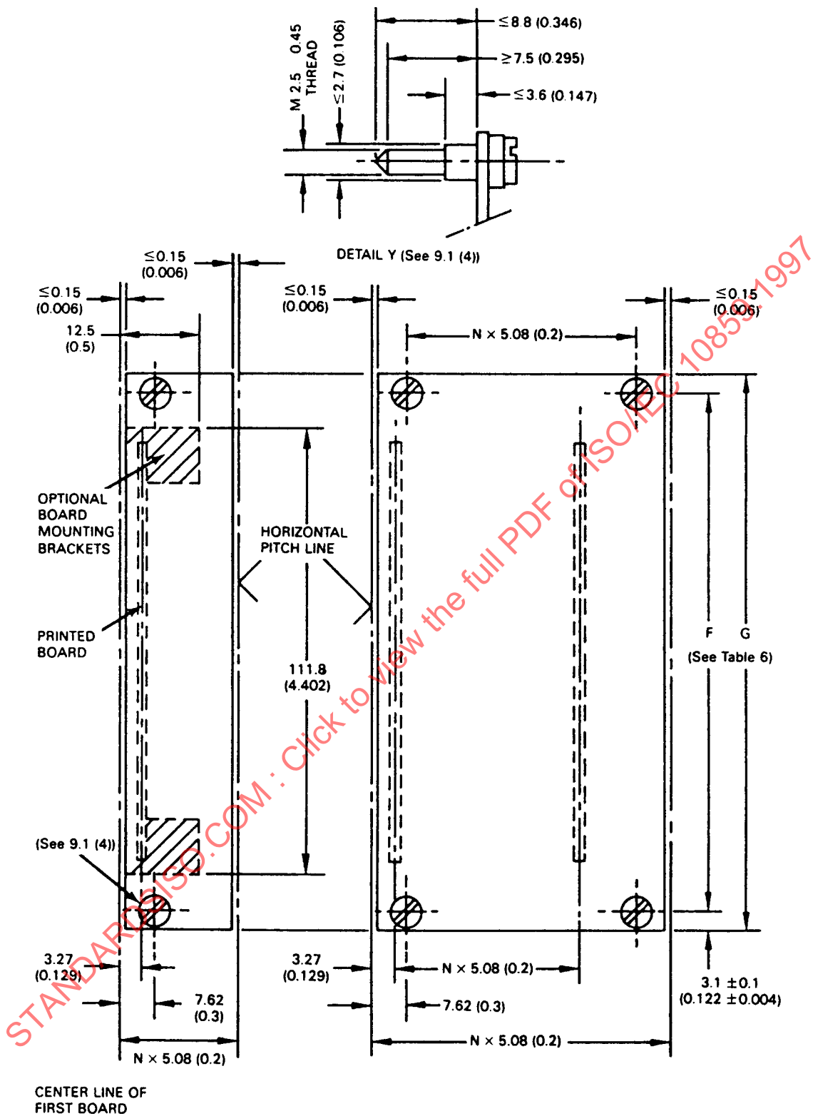
Figure 15 – Board type plug-in unit front panel
