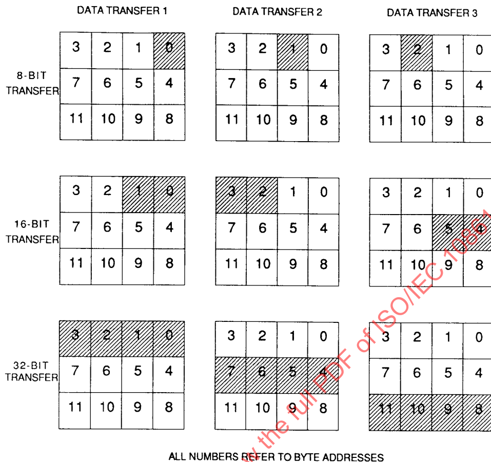
Figure 6.3-14—Block diagram of sequential data transfers in memory space
