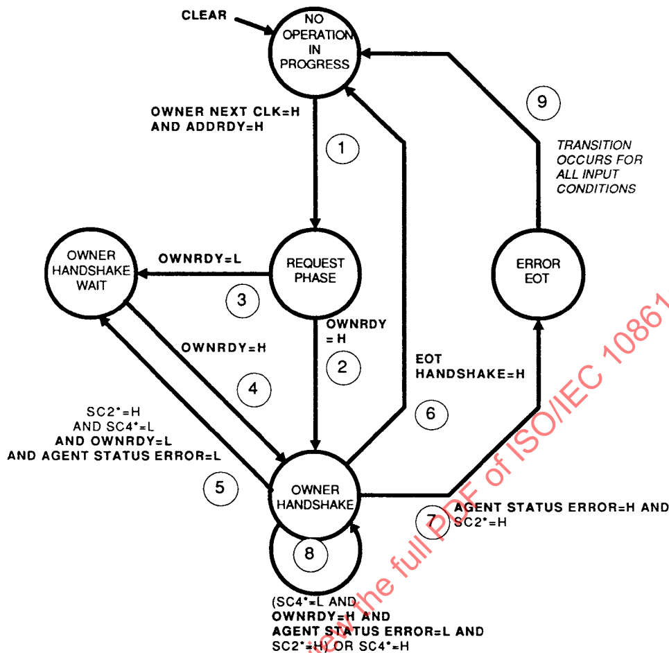
Figure 6.6-4 — State-flow diagram for requesting agents in a transfer operation
