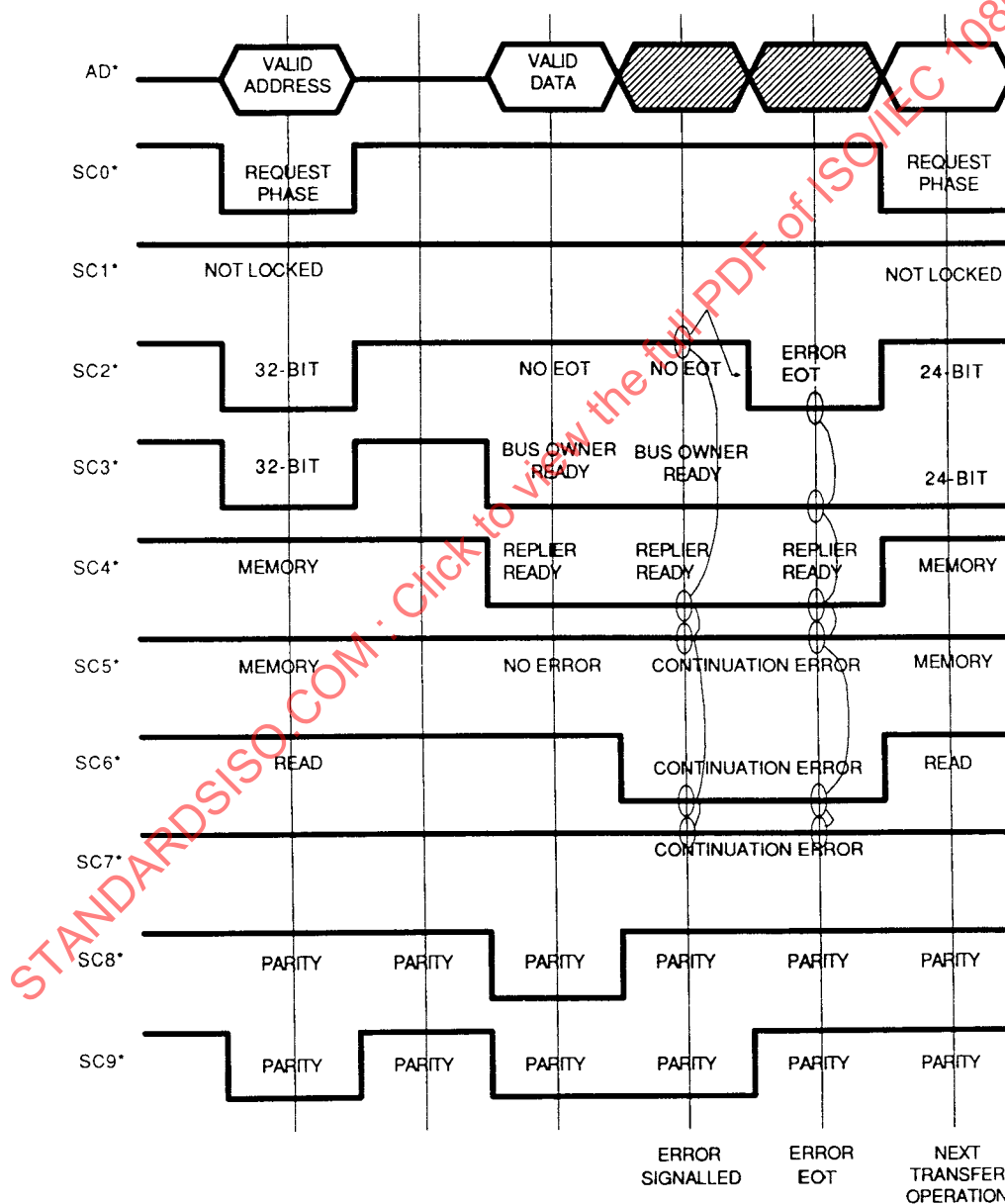
Figure 6.3-12—Timing sequence for continuation error
