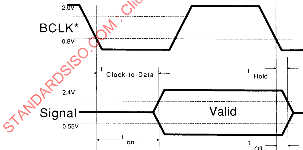
Figure 7.2-3—Driver timing parameters
