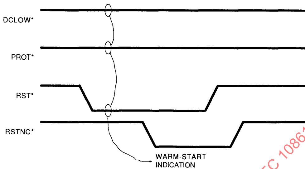
Figure 6.5-2—Warm-start reset sequence
