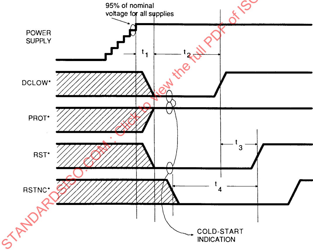
Figure 7.2-5 — Cold-start timing parameters
