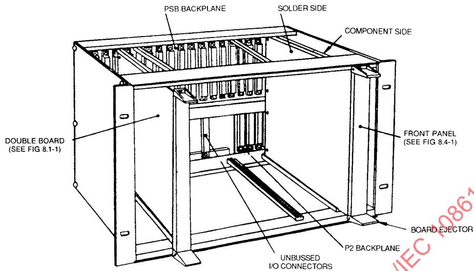
Figure 8.1-3 — Typical subrack
