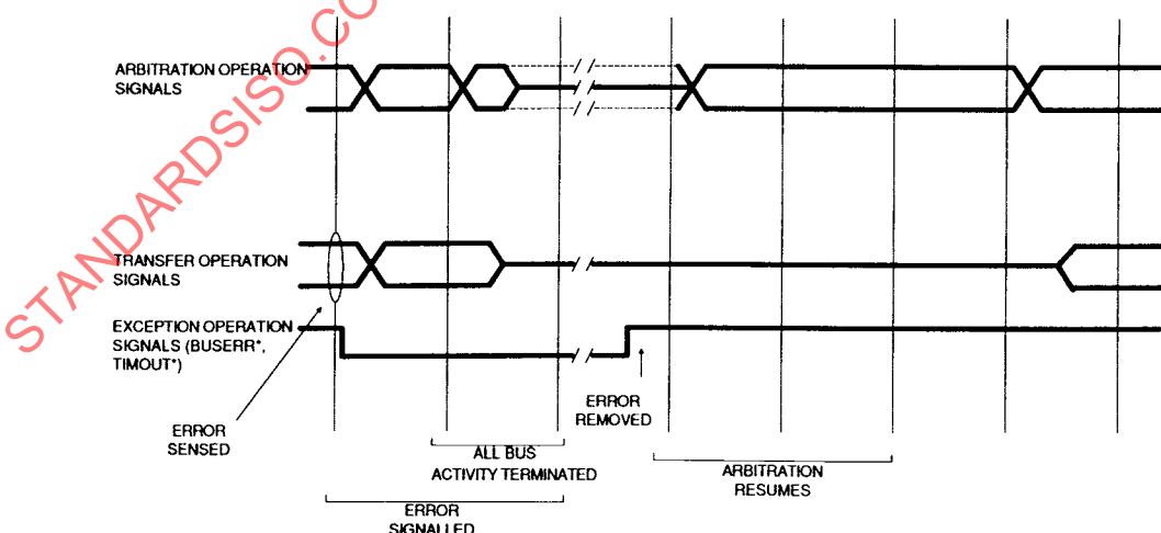
Figure 6.4-1 — Exception cycle signal relationships
