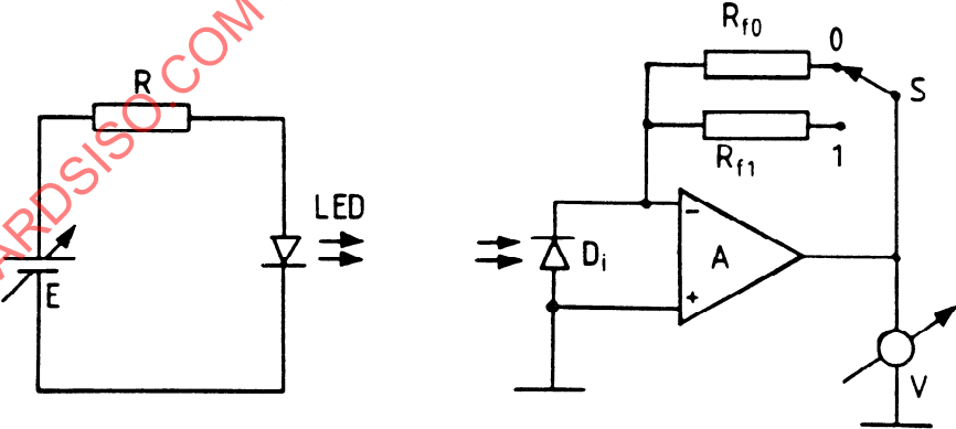
Figure B.2 - Electronic circuitry
