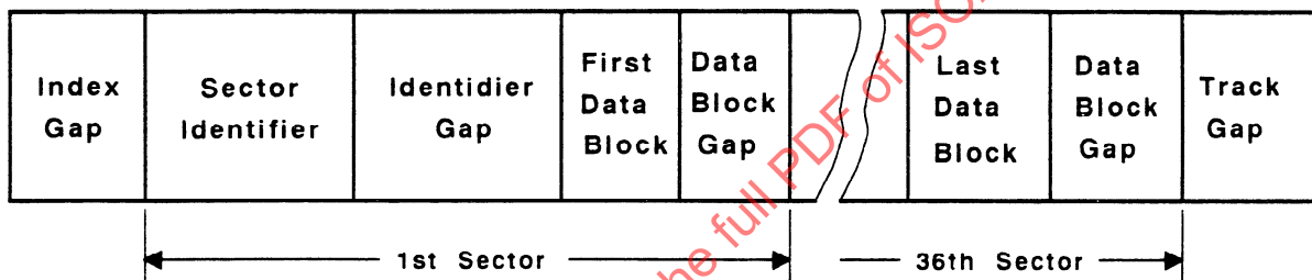
Figure 3 - Track layout
