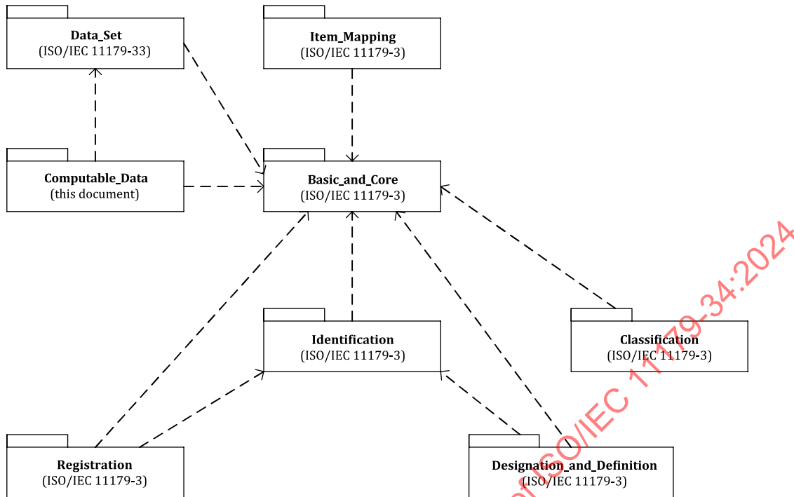
Figure 1 — Package dependencies
