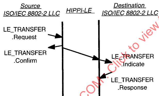
Figure 3 – Data transfer service primitives
