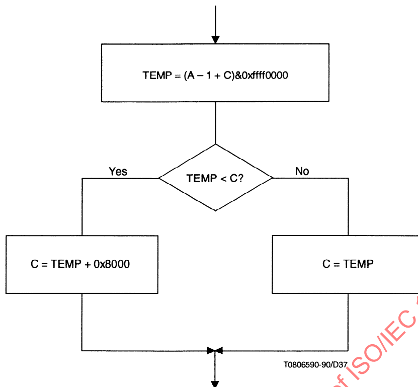
Figure 29 – Flow diagram for the procedure CLEARBITS
