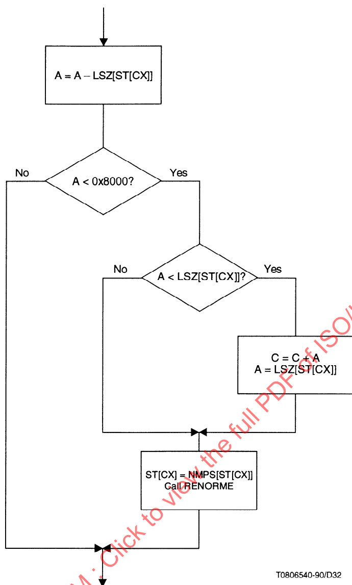
Figure 24 – Flow diagram for the procedure CODEMPS
