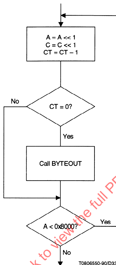
Figure 25 – Flow diagram for the procedure RENORME
