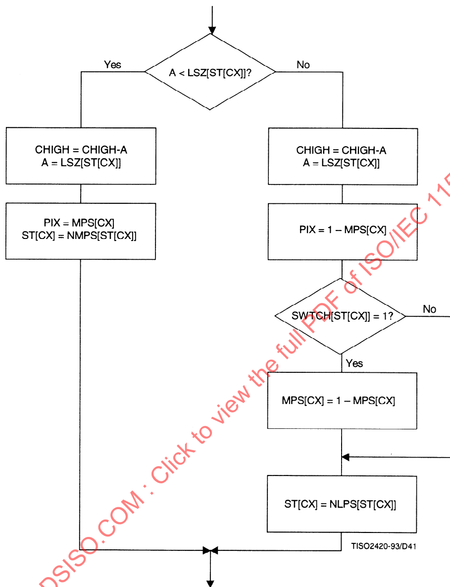
Figure 33 – Flow diagram for the procedure LPS_EXCHANGE
