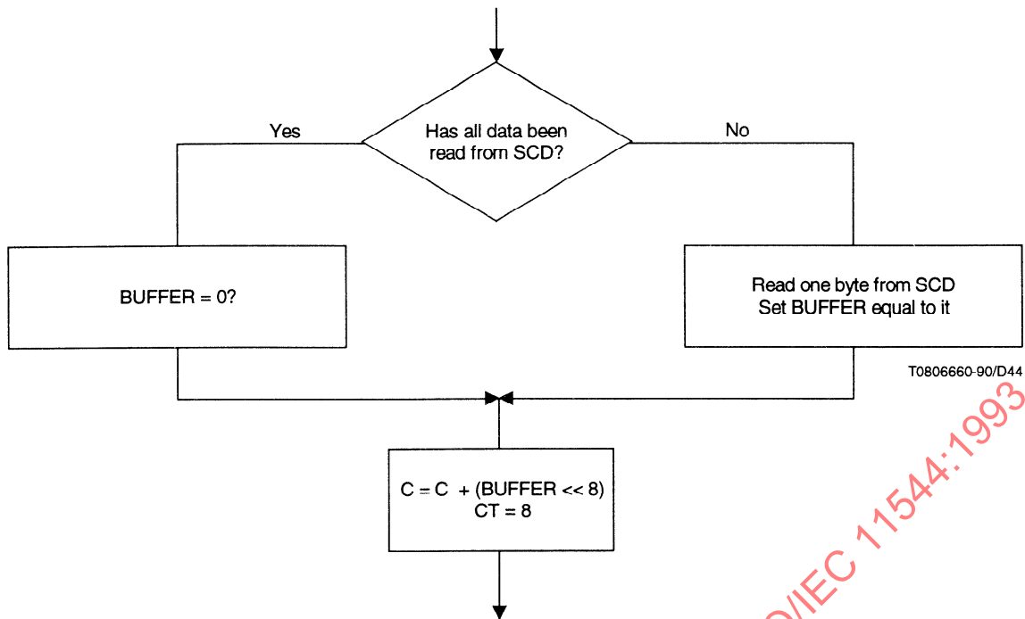
Figure 36 – Flow diagram for the procedure BYTEIN
