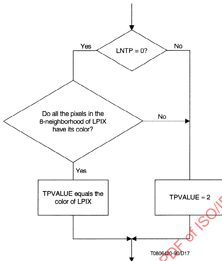
Figure 9 – Processing to determine TPVALUE
