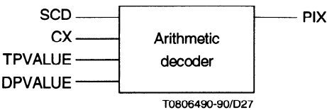
Figure 19 – Decoder inputs and outputs
