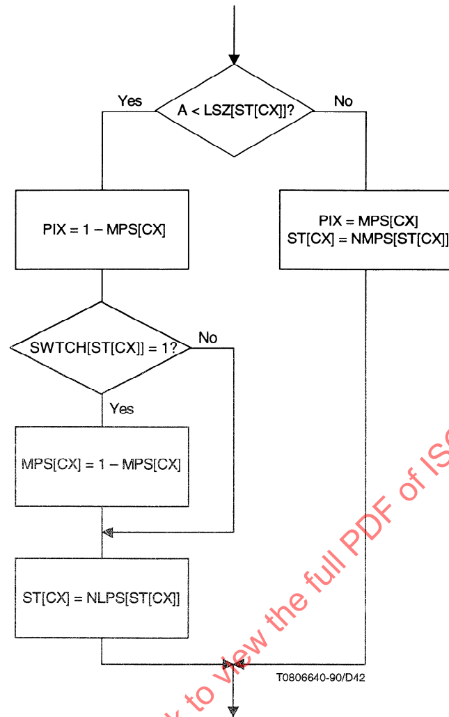
Figure 34 – Flow diagram for the procedure MPS_EXCHANGE
