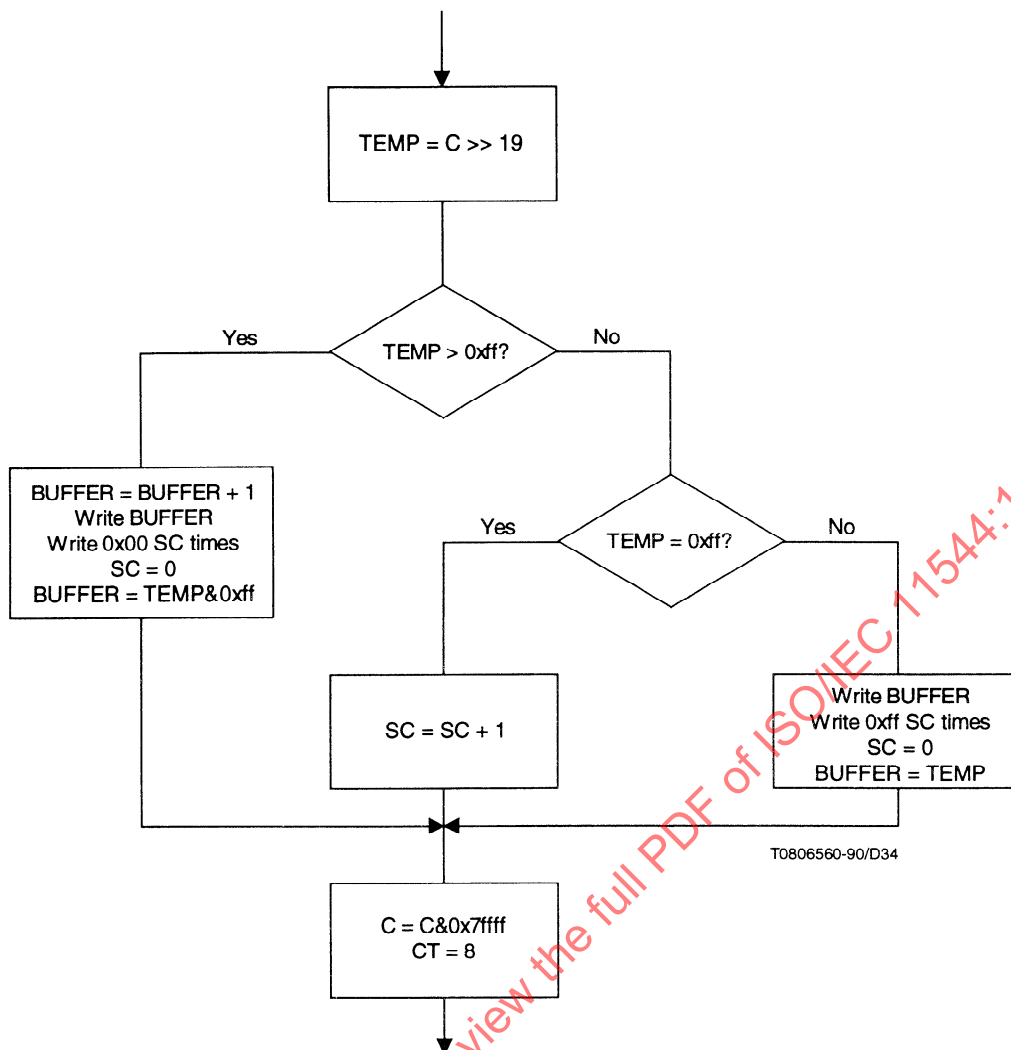
Figure 26 – Flow diagram for the procedure BYTEOUT
