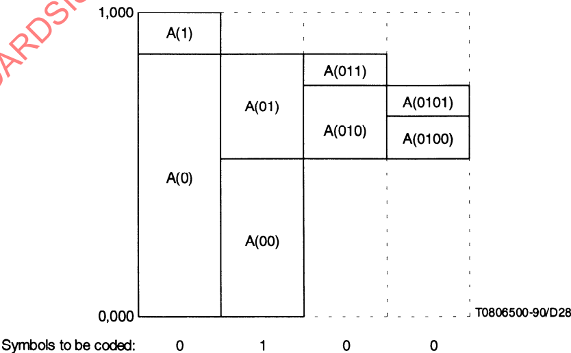
Figure 20 – Interval subdivision
