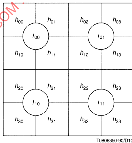
Figure 2 – High- and low-resolution pixels in two-dimensional graphic
