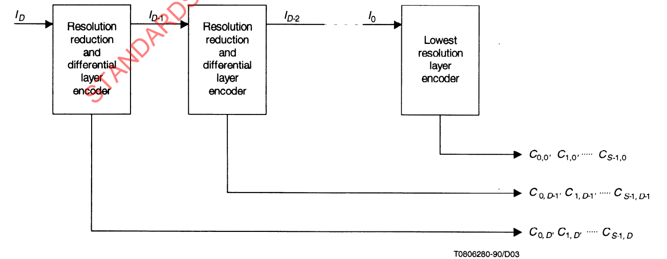
Figure 0.3 – Decomposition of encoder
