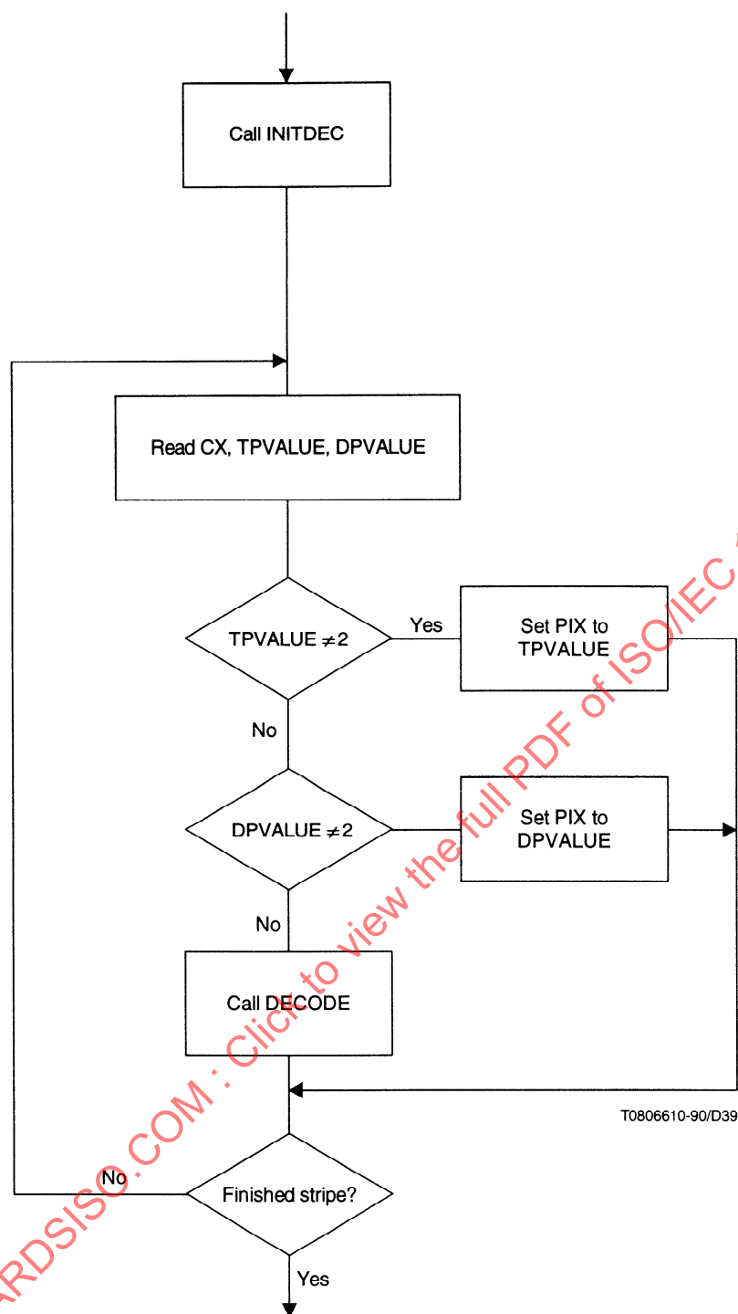
Figure 31 – Decoder flow diagram
