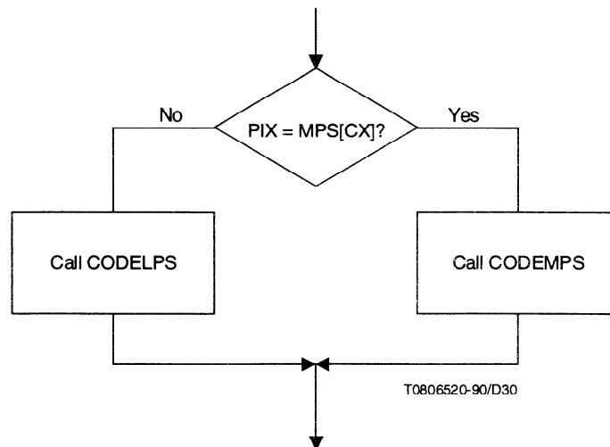
Figure 22 – Flow diagram for the procedure ENCODE
