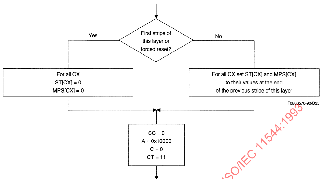
Figure 27 – Flow diagram for the procedure INTENC
