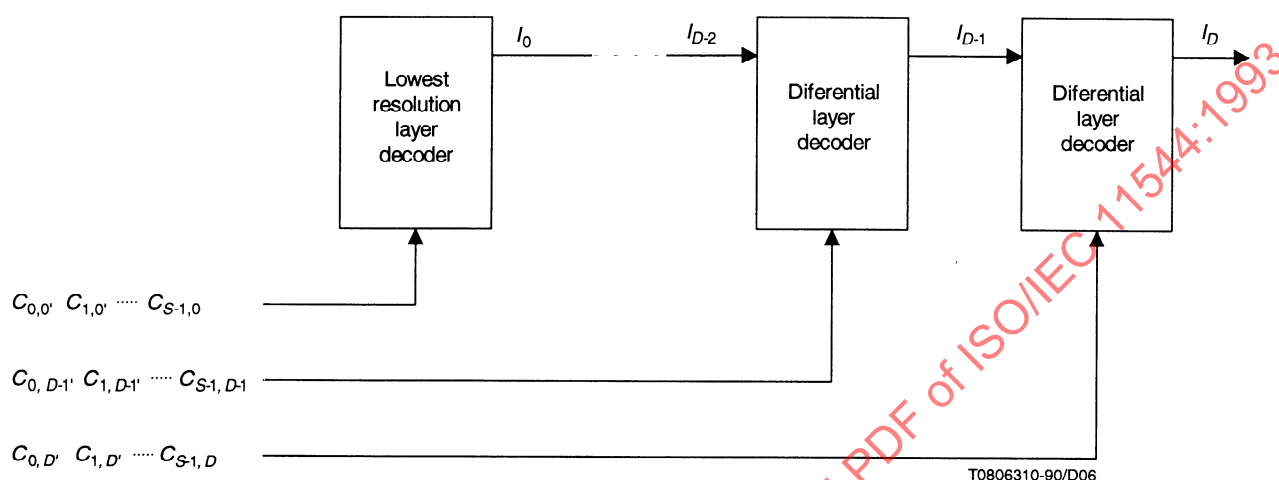
Figure 0.6 – Decomposition of decoder
