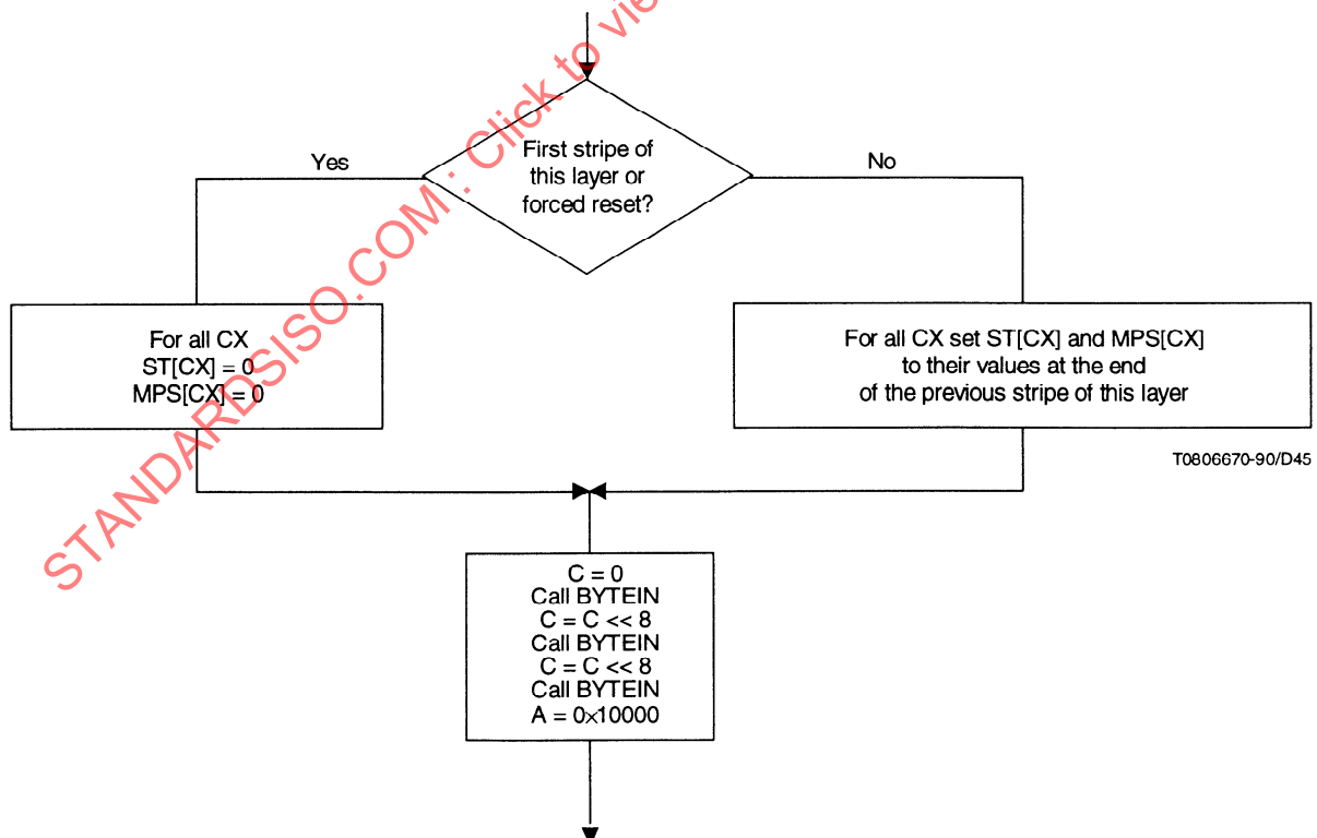
Figure 37 – Flow diagram for the procedure INITDEC
