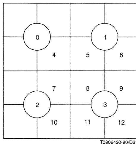
Figure 13 – Labeling of pixels used by DP
