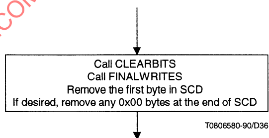
Figure 28 – Flow diagram for the procedure FLUSH
