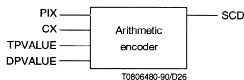
Figure 18 – Encoder inputs and outputs
