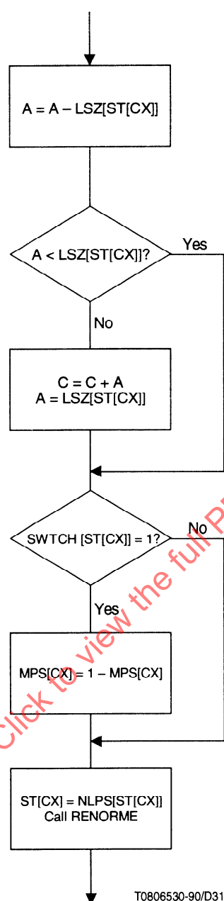
Figure 23 – Flow diagram for the procedure CODELPS
