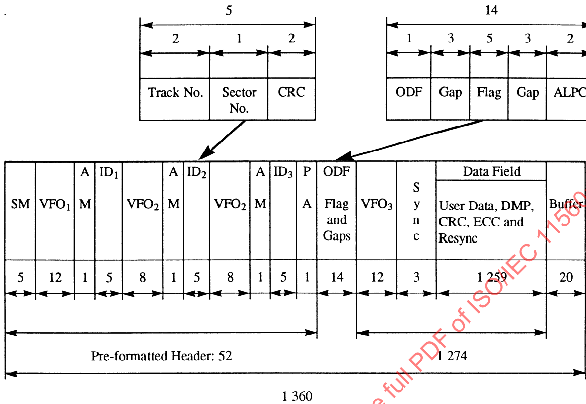
Figure 22 - Sector format for 1 024 user byte
